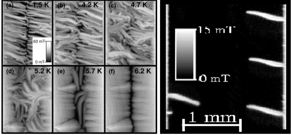
Figure 1.9: On the left: magnetic flux distribution of a Nb thin film of thickness 0.5 \mu\text{m} after zero-field cooling and for a magnetic field of 40 mT and different temperatures. The critical temperature is T_c \sim 9.2\text{K} . On the right: finger-like patterns in a 0.5 \mu\text{m} film of Nb at T = 4.2 \text{ K} and a field of 6.8 mT. After [14].
