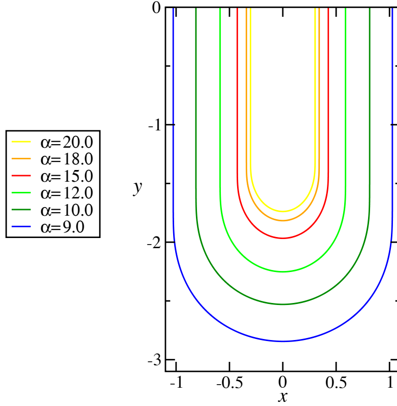
Figure 2.9: Fingers shapes in the case with smooth f(j, T) for different values of the coefficient \alpha for a velocity v_0 = 1.43 in our dimensionless variables, j = 0.92 , \tau = 10^{-1} and j_1 = 0.004 .
