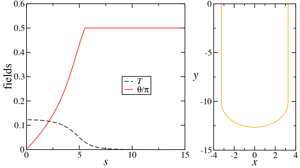
Figure 2.4: Plot of the profile of the angle \theta and the temperature T(s) as a function of the arclength s (on the left) and finger shape (on the right) for fixed parameters \tau = 0.1 , \alpha = 3.7 and the value found for the tip velocity v_0 = 1.07 .
