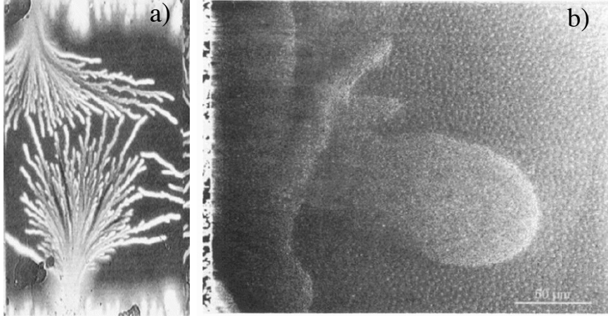
Figure 1.1: Examples of vortex patterns in type II superconductors. a) On the left dendritic patterns of vortices with branchlike structures in a Nb film of 0.5\ \mu\text{m} . The sample is at a temperature of 5.97\ \text{K} and the external field is 135\ \text{Oe} . After [10]. b) On the right droplet-like patterns observed with the decoration technique in a NbSe 2 single crystal at 5\ \text{mT} . Inside the droplet the density of vortices is higher, whereas in the outer region, where vortices are more visible, the density is lower. After [17, 18].
