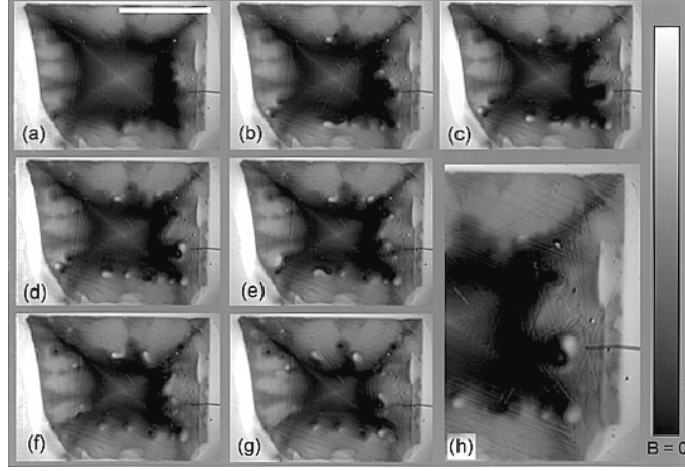
Figure 1.11: “Turbulent” behavior observed at the boundaries between vortices and antivortices in a \text{YBa}_2\text{Cu}_3\text{O}_{7-\delta} single crystal at a temperature of 65 K. The sequence shows the time development after a) 10 s, b) 20 s, c) 30 s, d) 40 s, e) 60 s, f) 90 s and g) 150 s. After [24].
