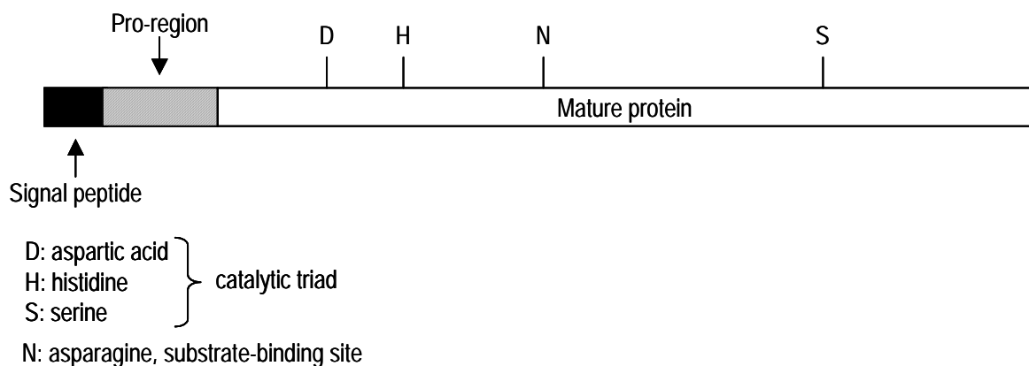
Figure 3. Schematic representation of the structure of the AIR3 protein.
