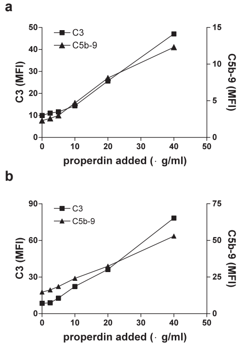
Figure 5 Dose-dependent effect of properdin on complement deposition
