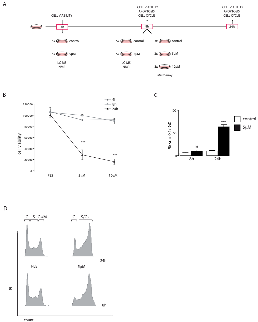
Figure S1. Cisplatin does not lead to cell death at 4 h and 8 h of treatment, but causes cell cycle arrest. (A) Schematic representation of the experiments. (B) Cell viability measured by ATPite in ES cells after treatment with 5 µM and 10 µM cisplatin at 4 h, 8 h and 24 h of treatment. (C) Apoptosis measured by FACS analysis after 8 h and 24 h of treatment with 5 µM cisplatin. (D) Cell cycle profile after 8 h and 24 h treatment with PBS or 5 µM cisplatin.
