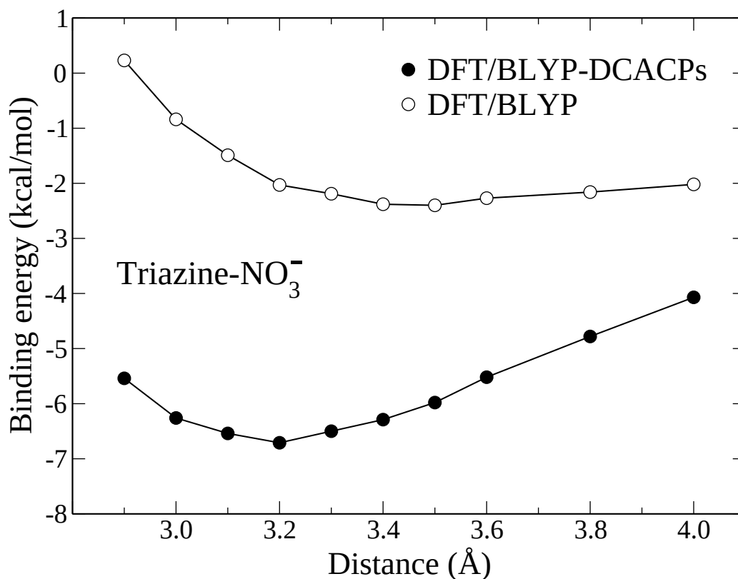
Figure 5.2: Binding energy of the triazine- \text{NO}_3^- system in the parallel geometry as a function of the distance between the centroid of the triazine ring and the nitrogen atom of \text{NO}_3^- . The curves are computed within DFT/BLYP with and without the DCACPs.
