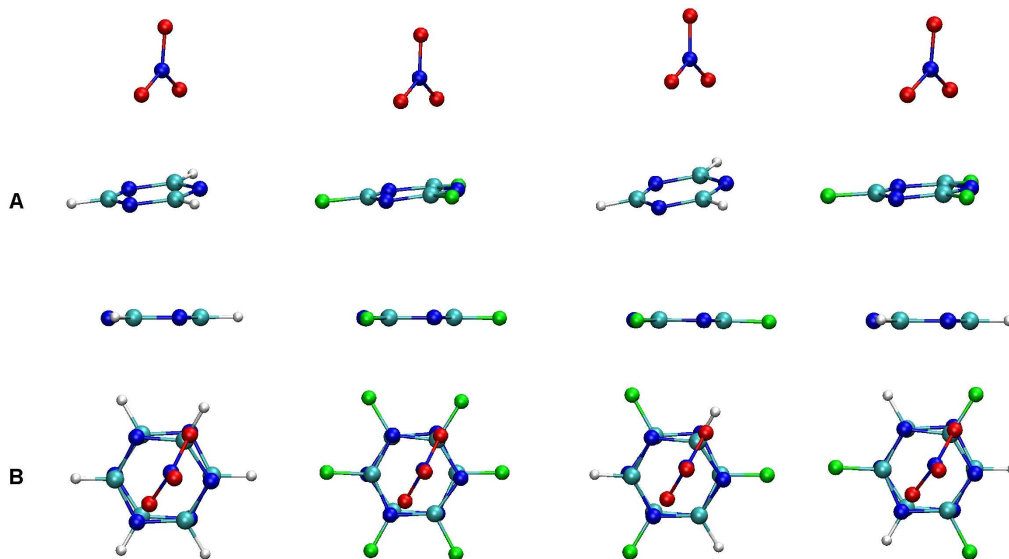
Figure 5.5: Side (A) and top (B) view of four different \pi - \pi complexes interacting with \text{NO}_3^- . From left to right, we show two triazine (TAZ) rings at 60°, two trifluorotriazine (TFT) at 60°, and the two mixed systems, TFT-TAZ and the TAZ-TFT. The TFT-TAZ and TAZ-TFT complexes have the TFT and TAZ ring closer to the \text{NO}_3^- , respectively.
