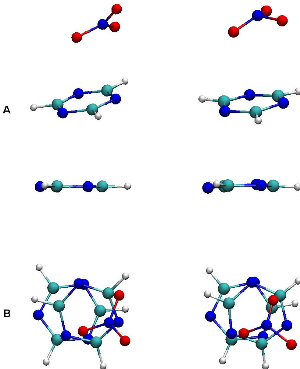
Figure 5.4: Side (A) and top (B) view of the triazine-triazine- \text{NO}_3^- complex as obtained within DFT/BLYP-DCACP (left) and experimentally [109] (right). In the top view, the bottom ring is parallel to the page.
