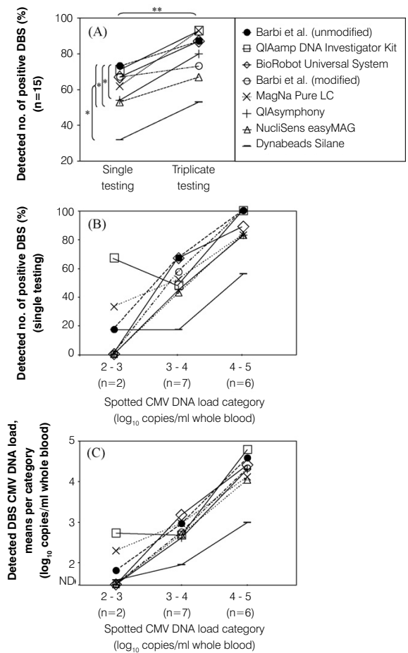
Figure 1 (A) Qualitative results of CMV DNA detection from DBS of the extraction methods tested, demonstrating the effect of triplicate testing on sensitivity. Left: single testing, right: triplicate testing (DBS was counted positive when \geq 1 of the triplicates was positive). * P \leq 0.05 , ** P \leq 0.01 . (B) Qualitative results of CMV detection from DBS of the extraction methods, per spotted CMV DNA load category, after single testing. (C) Quantitative results of CMV DNA detection from DBS of the extraction methods tested, per spotted CMV DNA load category. Depicted are detected mean CMV DNA loads of triplicates per category. DBS, dried blood spot; CMV, cytomegalovirus.
