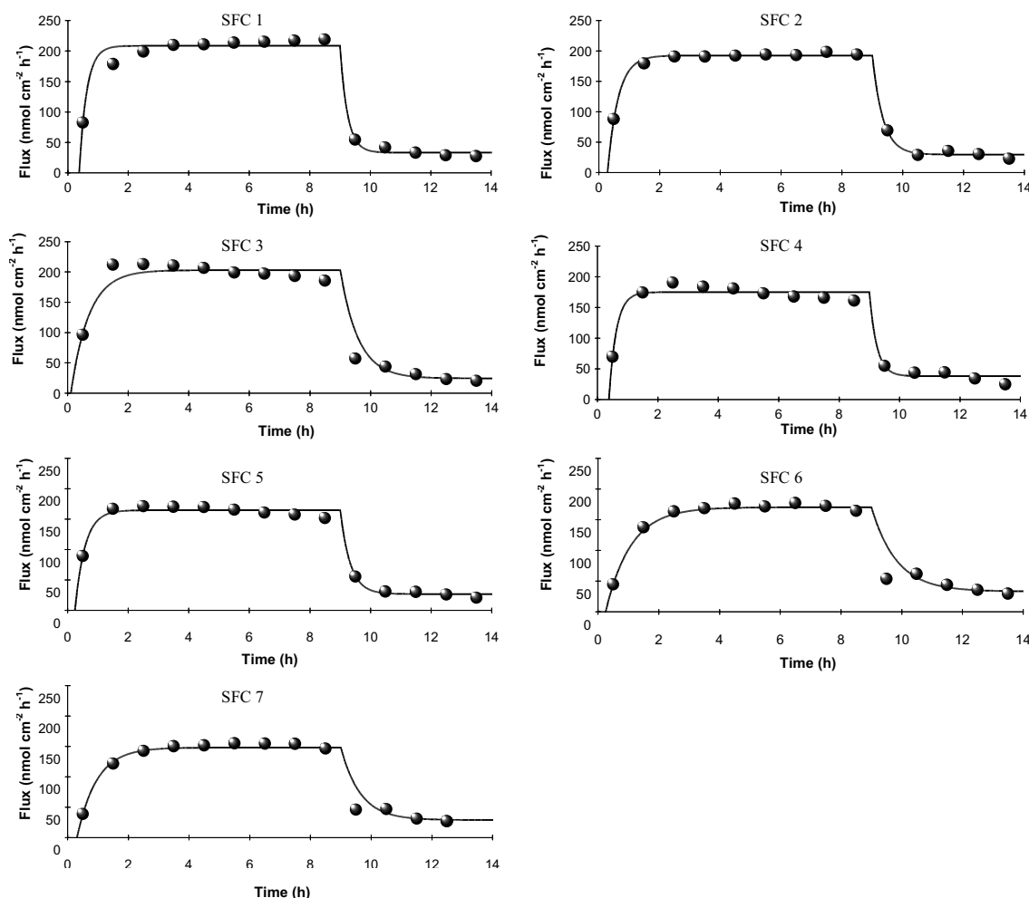
Fig. 6. The individual R-apomorphine (PBS group) transport during 9 hours iontophoresis and 6 hours post iontophoresis (filled circles) and the individual model prediction curves based on model 1 (solid line).
