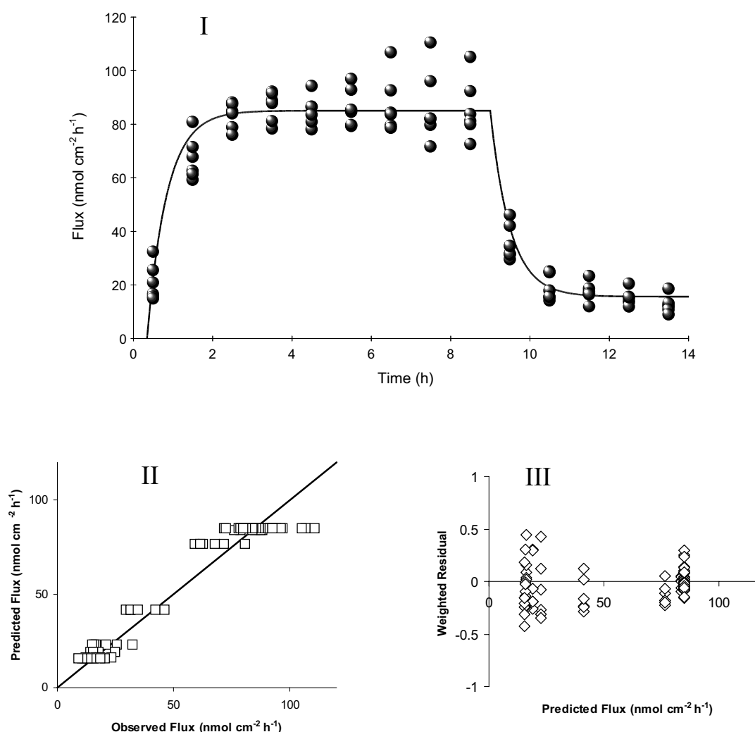
Fig. 3. The fitting result (I) and the evaluation of the predicted flux versus observed flux (II) and the weighted residual sum of square versus predicted flux (III) based on the naïve pooling approach of the data-set of R-apomorphine transport from PBS group during iontophoresis and in post iontophoretic period using model 1.
