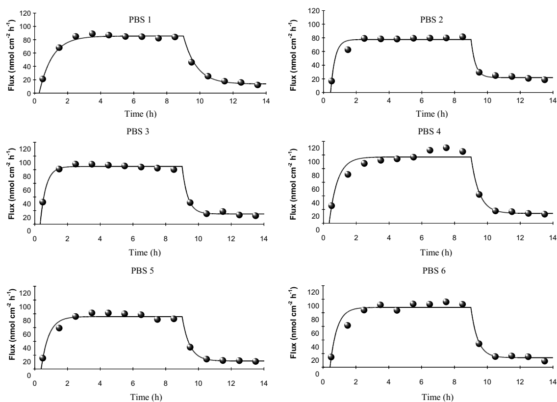
Fig. 6. The individual R-apomorphine (PBS group) transport during 9 hours iontophoresis and 6 hours post iontophoresis (filled circles) and the individual model prediction curves based on model 1 (solid line).
