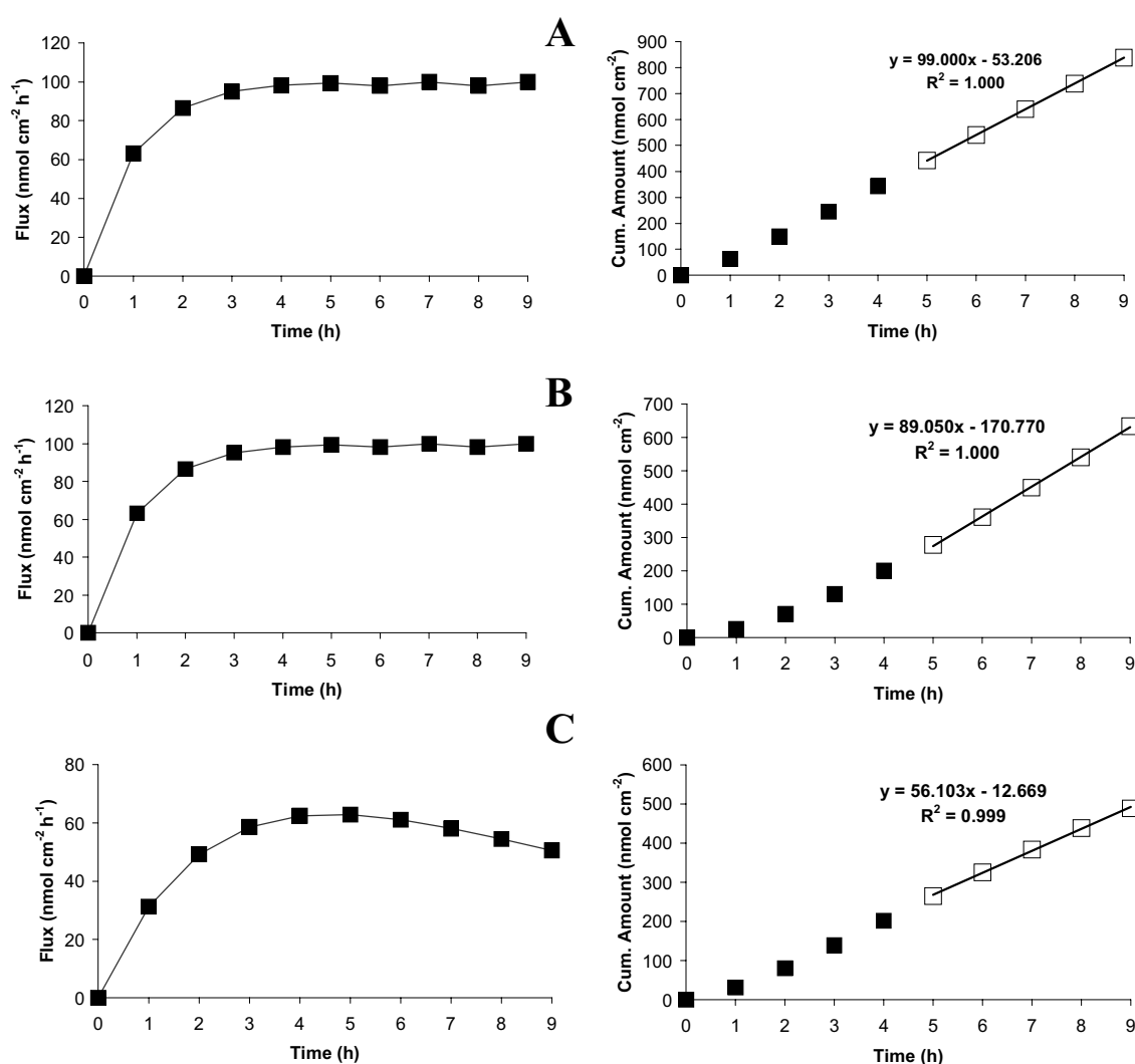
Fig. 1. The correlation of the flux versus time profiles to the transported cumulative amount versus time profiles. Although only in part A the real steady-state is achieved, the transported cumulative amount profiles in parts B and C also exhibit linear correlation to the time, demonstrating that linearity in the transported cumulative amount does not always indicate a steady-state achievement.
