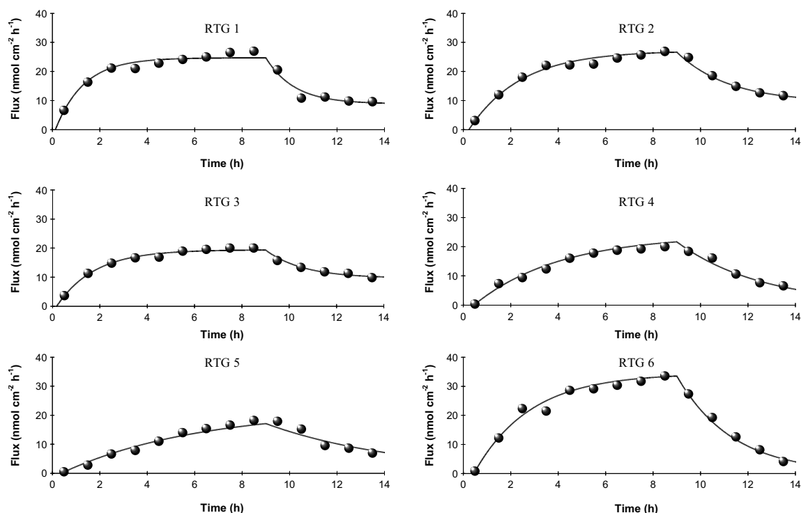
Fig. 8. The individual rotigotine transport during 9 hours iontophoresis and 6 hours post iontophoresis (filled circles) and the individual model prediction curves based on model 1 (solid line).
