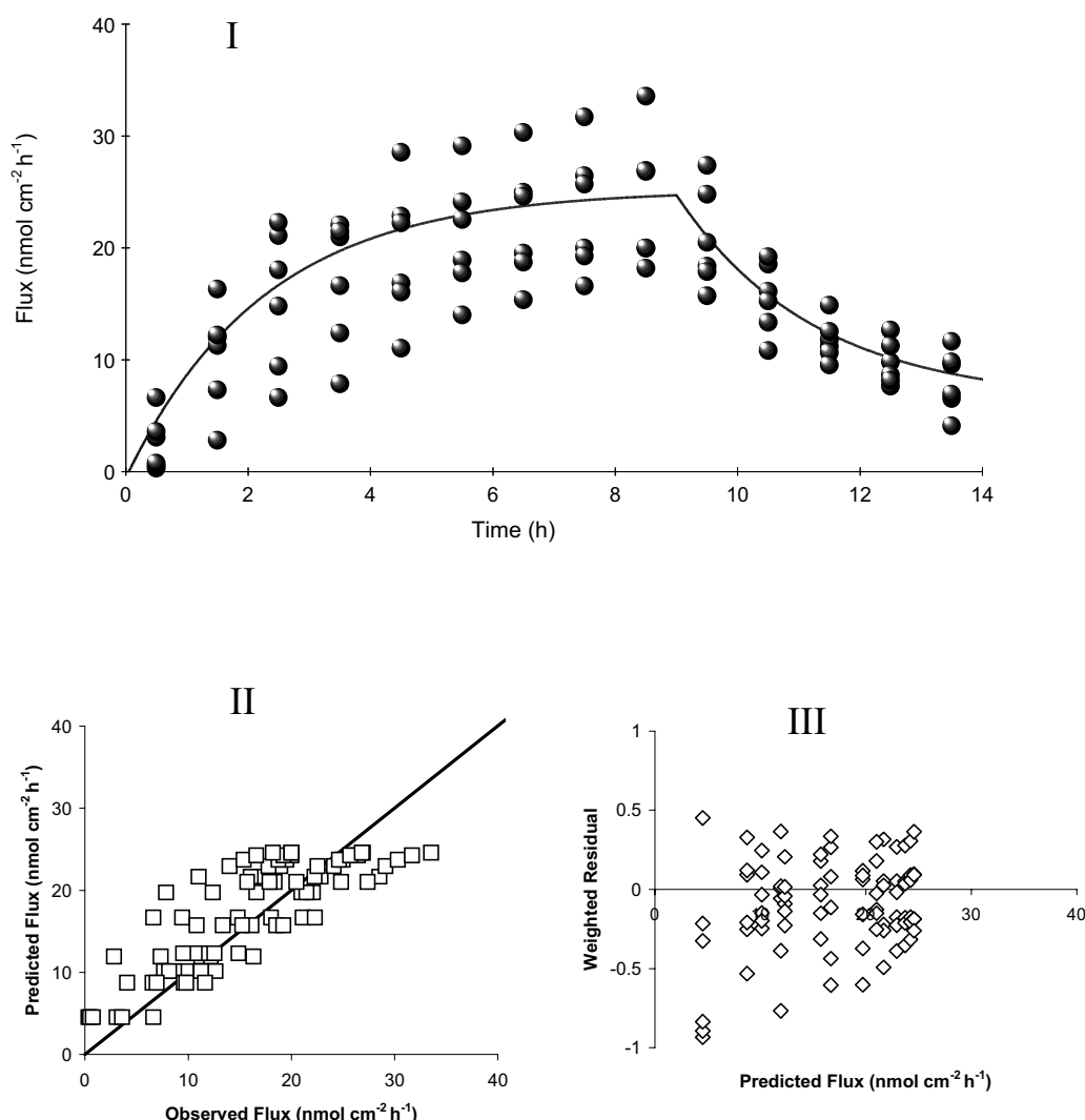
Fig. 5. The fitting result (I) and the evaluation of the predicted flux versus observed flux (II) and the weighted residual sum of square versus predicted flux (III) based on the naïve pooling approach of the data-set of rotigotine transport during iontophoresis and in post iontophoretic period using model 1.
