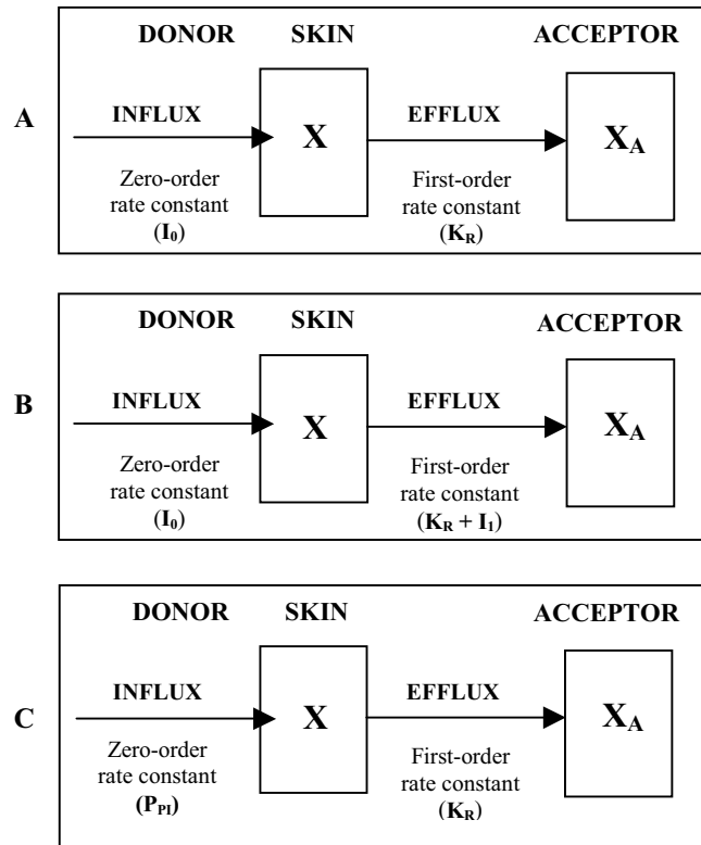
Fig. 2. Schemes of compartmental mass transfer during iontophoretic periods (A and B) and post iontophoretic period (C). Legends: X: Drug amount in the skin compartment, X A : Drug amount in the acceptor compartment
