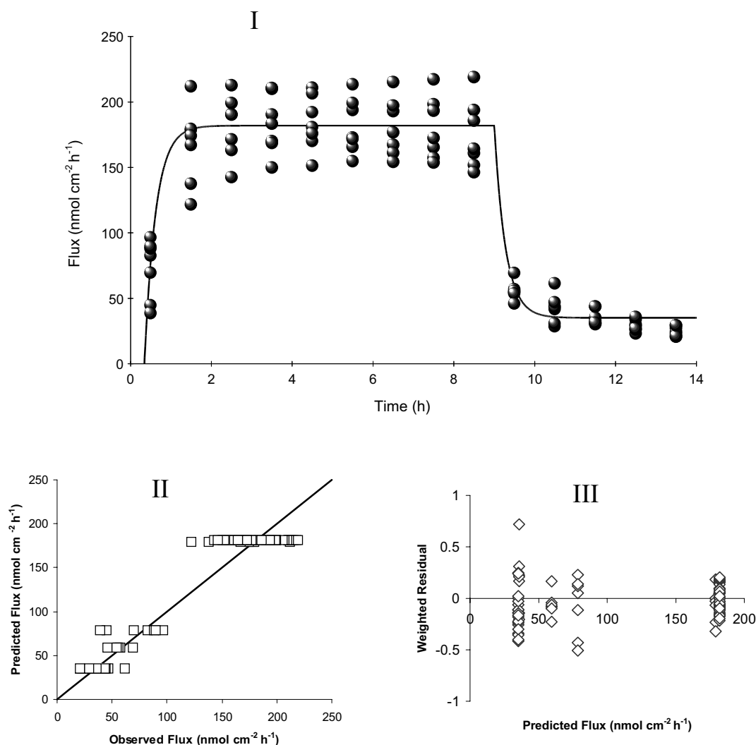
Fig. 4. The fitting result (I) and the evaluation of the predicted flux versus observed flux (II) and the weighted residual sum of square versus predicted flux (III) based on the naïve pooling approach of the data-set of R-apomorphine transport from SFC group during iontophoresis and in post iontophoretic period using model 1.
