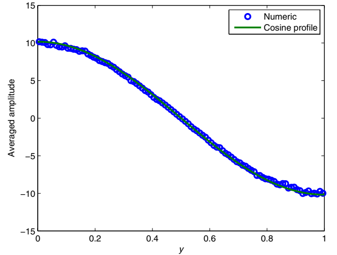
FIG. 4. The lowest-frequency mode is shown for a single matrix with N = 500\,000 , \varepsilon = 0.1 , in two dimensions. The amplitudes are binned along one of the sides of the square in which the points are randomly chosen, and the graph shows the sum of amplitudes in each bin. While the eigenmode itself is not a simple plane wave, after coarse graining in this way, one obtains a cosine profile, precisely as would be obtained in an ordered system.
