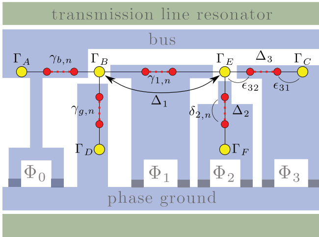
FIG. 2. (Color online) Transmon circuit for demonstration of non-Abelian statistics (Ref. 8). Two large superconducting islands (bus and ground) are used in the readout of the topological qubit and three smaller superconducting islands are needed for braiding. The nanowires form a \pi -shaped circuit hosting six computational Majoranas, \Gamma_A, \Gamma_B, \dots, \Gamma_F . A strong disorder can induce accidental Majorana modes \gamma_{k,n} , where k labels the island and n the accidental Majorana mode within the island. These accidental modes are coupled to each other with couplings \delta_{k,n} , and the accidental Majoranas closest to the end of the wires are coupled to the corresponding end states with \epsilon_{k1} and \epsilon_{k2} .
