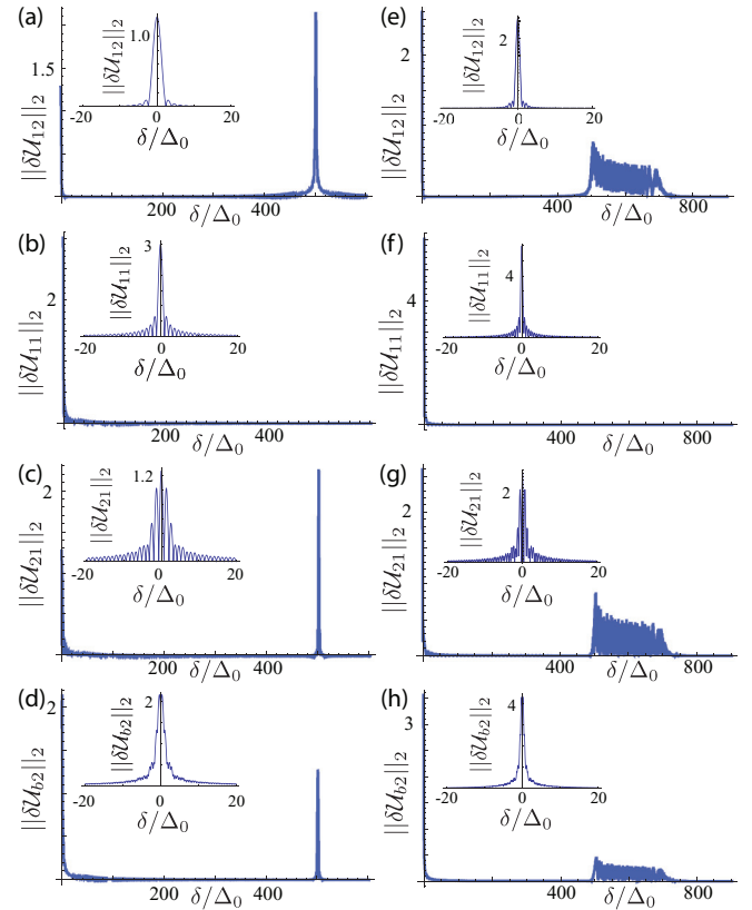
FIG. 4. (Color online) Errors occurring during the braiding cycle can be estimated by \epsilon_{ki} \|\delta \mathcal{U}_{ki}\|_2 / \Delta_0 [Eq. (6)], with four different types of corrections \|\delta \mathcal{U}_{ki}\|_2 , which are plotted as a function of \delta . These corrections, related to the two adiabatic cycles of Fig. 3(a),(b), are shown in panels (a)–(d) and (e)–(h), respectively. The insets show magnifications of the peaks around \delta = 0 . Away from the peaks the errors are efficiently suppressed. In all panels \Delta_{\text{max}} = 500\Delta_0 .
