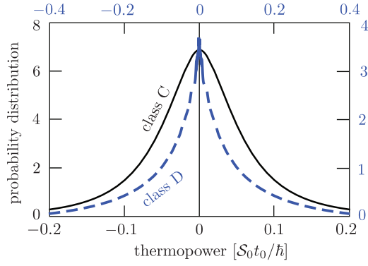
FIG. 5. (Color online) Probability distribution of the dimensionless thermopower p = \mathcal{S} \times \hbar / t_0 S_0 in symmetry class C (black solid curve, bottom and left axes), and in class D (blue dashed curve, top and right axes). These are results for the quantum dot of Fig. 2 connecting a single-channel point contact to the unpaired Majorana edge mode of a chiral p -wave superconductor (class D), or to the paired Majorana mode of a chiral d -wave superconductor (class C).
