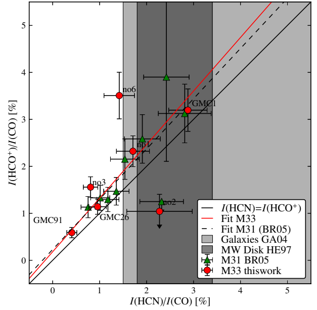
Fig. 5. Ratios of integrated intensities \text{HCO}^+ /CO vs. HCN/CO for M 33 (red points: this work) and for M 31 (green points: BR05). Upper/lower limits are denoted by arrows. Linear least squares fits to data from M 33 (red solid line) and M 31 (BR05, black dashed) are shown. Both fits exclude points with upper limits. The solid black line shows the angle bisector where I(\text{HCO}^+) = I(\text{HCN}) . The gray shaded areas display the range of the HCN/CO found in the disk of the Milky Way (MW) by (Helfer & Blitz 1997, HE97) (darker gray) and in a sample of normal spiral galaxies (GA04b) (lighter gray).
