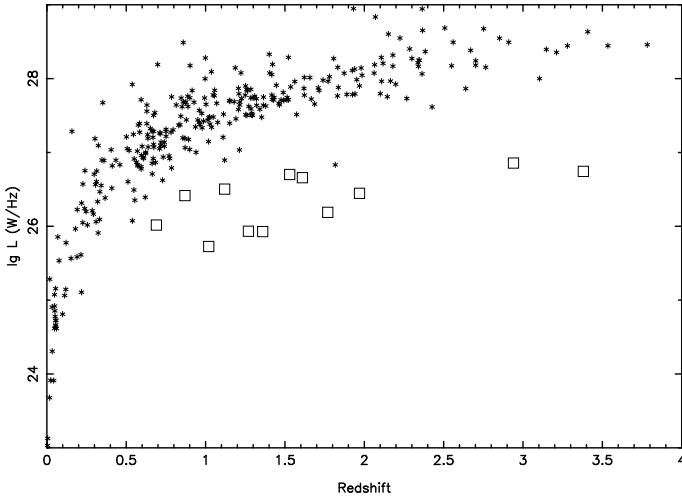
Fig. 7. The integrated 5-GHz radio luminosity ( \text{W Hz}^{-1} ) of the VLBI components as a function of the source redshift for the DEVOS sources with known redshift (squares) and the generally brighter radio-loud AGNs from Fomalont et al. (2000) (asterisks).
