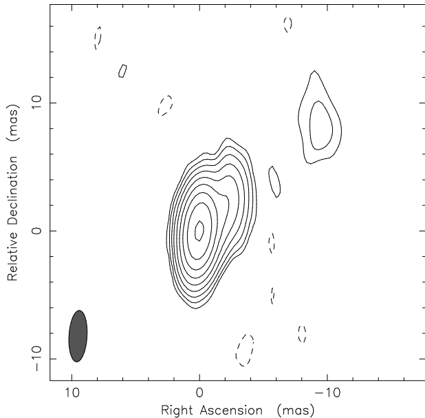
Fig. 4. Naturally weighted 5-GHz VLBI image of the reference source in Field B (J1623+3909). The lowest contours are drawn at \pm 0.3 mJy/beam. The positive contour levels increase by a factor of 2. The peak brightness is 85.4 mJy/beam. The restoring beam is 4.0 \text{ mas} \times 1.4 \text{ mas} at \text{PA} = -3^\circ 3 .
