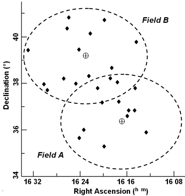
Fig. 1. Sketch of the celestial positions of the two phase-reference sources ( \oplus ) and the 26 programme sources. The borders of Fields A and B projected onto the right ascension–declination plane are indicated with dashed lines.
