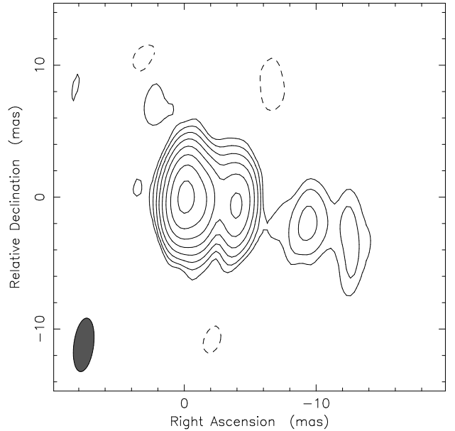
Fig. 3. Naturally weighted 5-GHz VLBI image of the reference source in Field A (J1616+3621). The lowest contours are drawn at \pm 0.5 mJy/beam. The positive contour levels increase by a factor of 2. The peak brightness is 81.4 mJy/beam. The restoring beam is 4.1 \text{ mas} \times 1.5 \text{ mas} at \text{PA} = -7.4^\circ . The coordinates are relative to the brightness peak. The Gaussian restoring beam is indicated with an ellipse in the lower-left corner.
