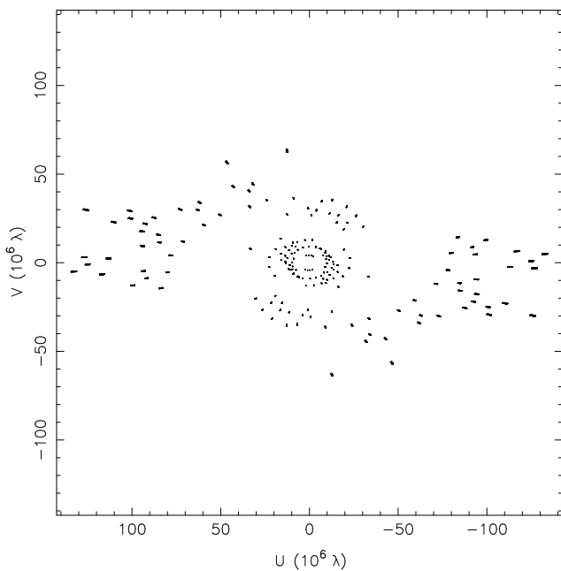
Fig. 2. The (u,v) -coverage of one of the target sources (J161252.4+355234) in our 5-GHz EVN observations.
