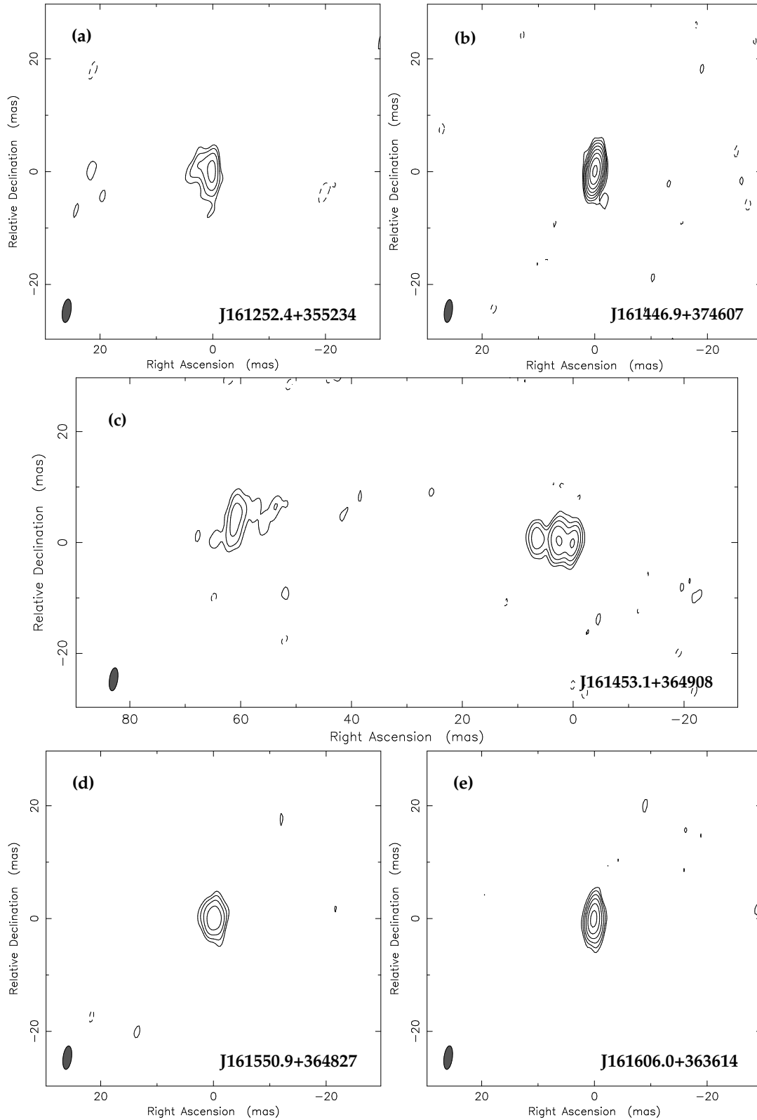
Fig. 5. Naturally weighted 5-GHz VLBI images of 24 programme sources. The image parameters (peak brightness, lowest contour level corresponding to 3\sigma image noise, Gaussian restoring beam size and orientation) are listed and explained in Table 2. The positive contour levels increase by a factor of 2. The coordinates are relative to the brightness peak for which the absolute coordinates are given in Table 1. The restoring beam is indicated with an ellipse in the lower-left corner.
