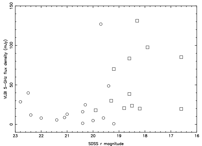
Fig. 6. The 5-GHz VLBI flux density (mJy) versus the SDSS r magnitude of the quasars detected with VLBI (this paper and Paper I). Spectroscopic redshifts are available for the objects marked with squares.
