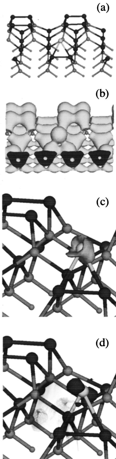
FIG. 2. The figure shows the geometry and some charge-density isosurfaces for an Au adatom located at the site D_1 of Fig. 1(a). (a) Atomic geometry, the As and Ga atoms are represented by black and gray spheres, respectively. The Au adatom is represented by the biggest gray sphere, the H atoms by the smallest spheres. (b) Total valence charge density, the isosurface corresponds to an electron density of 0.035 \text{ e/a.u.}^3 ; (c) D^- density (see the text), the isosurface corresponds to an electron density of 0.010 \text{ e/a.u.}^3 ; (d) D^+ density (see the text), the isosurface corresponds to an electron density of 0.010 \text{ e/a.u.}^3 .
