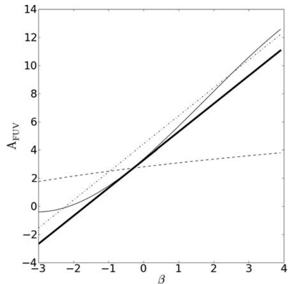
Figure 4. Different observational correlations between \beta and the attenuation at FUV wavelength, A_{FUV} . Thin solid line: equation (2) from Buat et al. (2005) combined with equation (5); dot-dashed line: Meurer et al. (1999); thick solid line: Wijesinghe et al. (2011); dashed line: this paper, equation (6) derived using the relationship between BD and \beta .
