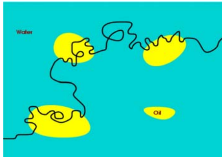
Fig. 1. An undirected copolymer in an emulsion
