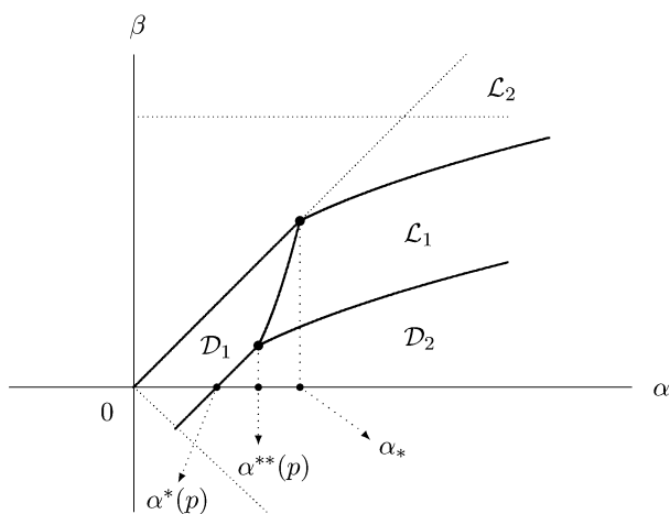
Fig. 9 Further details of the phase diagram for p < p_c sketched in Fig. 6. There are four phases, separated by three critical curves, meeting at two tricritical points
