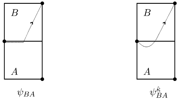
Fig. 5 Relevant paths for \psi_{BA} and \psi_{BA}^{\hat{\kappa}}
