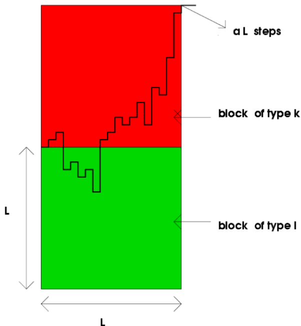
Fig. 4 Two neighbouring blocks and a piece of the path. The block that is crossed is of type k , the block that appears as its neighbor is of type l
