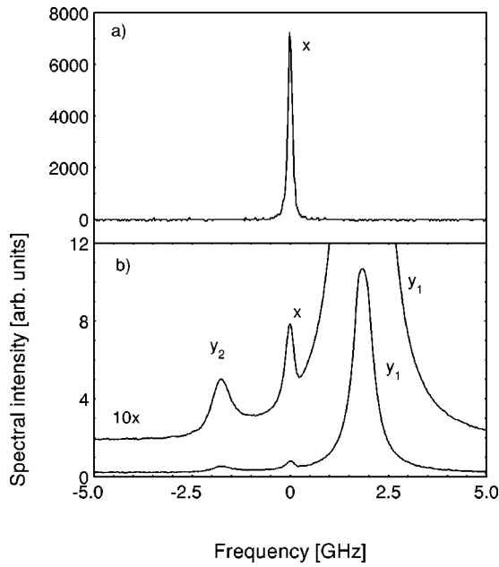
FIG. 3. Polarization-resolved optical spectra of VCSEL 1 at I = 9.0 mA, taking with a Fabry-Pérot interferometer. The x -polarized lasing peak, which dominates (a), is almost completely suppressed in the y -polarized spectrum of (b) (same arbitrary units). The latter shows the nonlasing peak at higher frequency and a weak FWM peak, as mirror image, at lower frequency.
