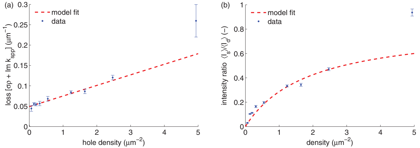
FIG. 4. (Color online) The loss and intensity ratio plotted as a function of hole density. (a) For all samples except the most dense, the loss increases linearly with hole density. The loss at zero hole density is the surface-plasmon absorption loss, which corresponds roughly to the literature value. (b) The surface-plasmon contribution \langle I_s \rangle relative to the direct contribution \langle I_d \rangle increases nonlinearly with hole density. Using only the vertical scale as a free parameter, the data can be reasonably fitted to theory.
