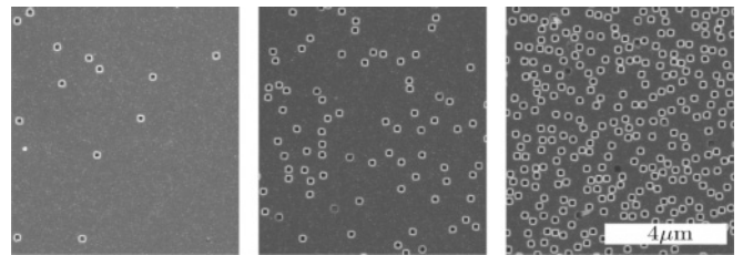
FIG. 1. SEM images of three of the nine studied samples. From left to right the hole density is 0.19, 1.2, and 4.9 \mu\text{m}^{-2} .
