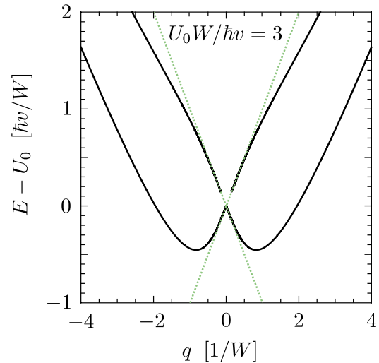
FIG. 4 (color online). Same as Fig. 3, but now showing the lowest channel modes in the fully quantum mechanical regime U_0W/\hbar v = 3 . The two minima at q = \pm 0.83W^{-1} each contribute independently an amount of 4e^2/h to the conductance.
