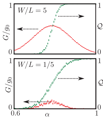
FIG. 6. (Color online) Average topological invariant Q (4.12) and longitudinal conductance G of a disordered quantum Hall sample for different aspect ratios as a function of the mixing angle \alpha .
