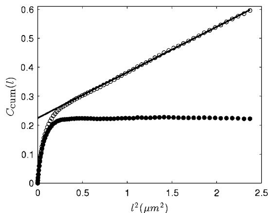
FIGURE 6 Experimentally obtained cumulative correlation function C_{\text{cum}}(l) . C_{\text{cum}}(l) was obtained for individual H-Ras (N17) molecules at the apical side of 3T3-A14 cells with a time-lag \Delta t of 20 ms (open circles, C_{\text{cum}}(l) ; solid line, linear fit of the long distance data yielded a concentration c \approx 0.16/\mu\text{m}^2 ; and solid circle, after subtraction of the correction term). Fit of the corrected data to Eq. 15 yielded \alpha = 0.90 \pm 0.02 , r_1^2 = 0.072 \pm 0.002 \mu\text{m}^2 , and r_2^2 = 0.012 \pm 0.0003 \mu\text{m}^2 .
