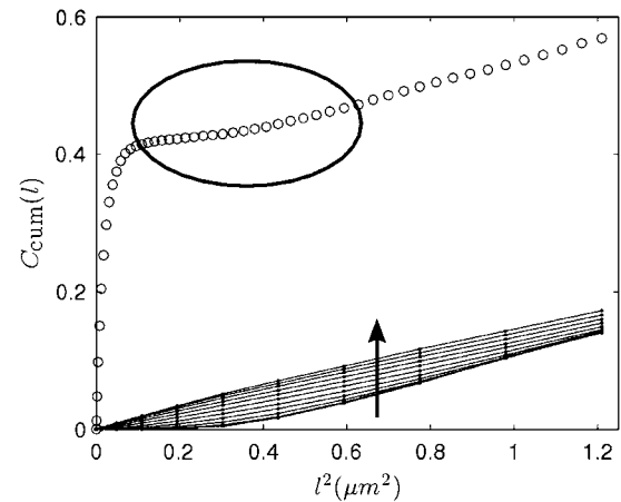
FIGURE 8 Correction for random spatial proximity of molecules at short distances and short time lag. The dip in the data obtained for individual H-Ras(N17) molecules at the apical side of 3T3-A14 cells taken at a time delay of 5 ms is due to diffraction (open circles, raw data; solid lines, pure spatial correlation for distances r from an arbitrary molecule; and r = 0 \mu\text{m} , 0.11 \mu\text{m} , 0.22 \mu\text{m} , \dots , 1.21 \mu\text{m} where r rises in the direction of the arrow).
