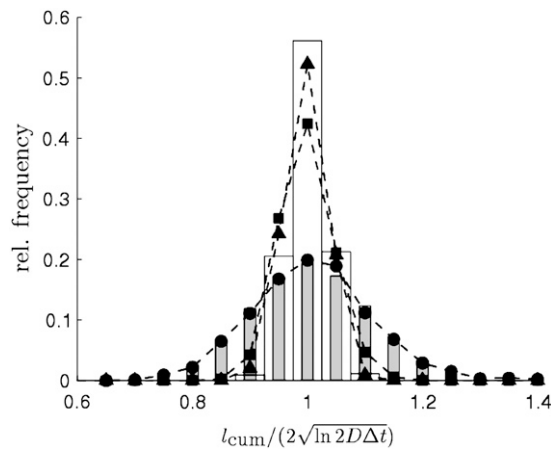
FIGURE 5 Distribution of l_{\text{cum}} from simulations including photobleaching. One-hundred image-pairs were analyzed at a concentration of 0.1/\mu\text{m}^2 , diffusion constant D = 1 \mu\text{m}^2/\text{s} , and time-lag \Delta t = 20 ms. (Triangle, p_{\text{dark}} = 0 ; square, p_{\text{dark}} = 0.4 ; circles, p_{\text{dark}} = 0.9 ; open bars, distribution as given by Eq. 13 with N = 500 ; and shaded bars, distribution as given by Eq. 13 with N = 50 .)
