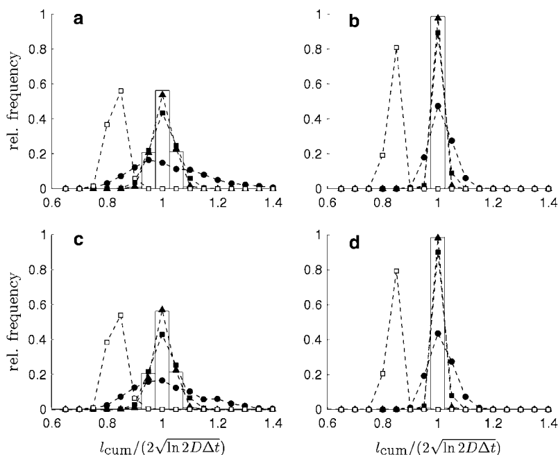
FIGURE 4 Distribution of l_{\text{cum}} from simulations. (a,b) Influence of molecule concentration at fixed D\Delta t = 1 \mu\text{m}^2/\text{s} and given number of images M = 100 (a), and M = 1000 (b) (solid triangle, c = 0.1/\mu\text{m}^2 ; solid square, c = 1/\mu\text{m}^2 ; solid circle, c = 10/\mu\text{m}^2 ; open square, same values as for the solid squares but without correction term; and bars, distribution as given by Eq. 13 with N = 500 for panel a and N = 5000 for panel b). (c,d) Influence of rising diffusion constant for constant c = 1/\mu\text{m}^2 and given number of images M = 100 (c), and M = 1000 (d). (Solid triangle, D\Delta t = 0.1 \mu\text{m}^2/\text{s} ; solid square, D\Delta t = 1 \mu\text{m}^2/\text{s} ; solid circle, D\Delta t = 10 \mu\text{m}^2/\text{s} ; open square, same values as for the solid squares but without correction term; and bars, distribution as given by Eq. 13 with N = 500 for panel c and N = 5000 for panel d.)
