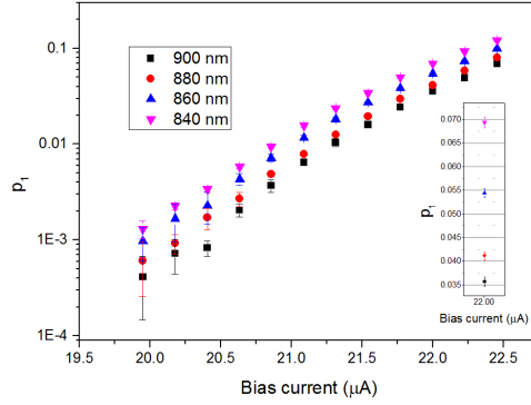
Figure 4.11: Quantum detector tomography of a superconducting single-photon detector at a series of narrowly spaced wavelengths
