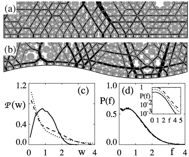
FIG. 4. (a), (b) Packing and force networks in a weakly polydisperse packing near a flat bottom (a) and a curved bottom (two circle segments of radius 20 glued together) (b). (c) Distribution of weights \mathcal{P}(w) on the flat bottom (solid line), convex curved bottom (dashed line), and the concave curved bottom (dotted line). The various shapes originate from the corresponding \{\rho_0, \rho_1, \rho_2\} : \{0.00, 0.10, 0.90\} , \{0.02, 0.39, 0.58\} , and \{0.04, 0.46, 0.50\} , respectively. (d) P(f) in the bulk ( h ranging from 10 to 20) for the flat, convex, and concave bottoms; the inset shows the P(f) 's on a log-lin scale (the curves are offset for clarity).
