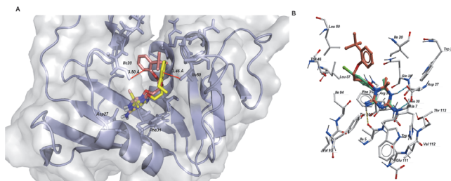
Fig 4. Binding mode of BRL-7980SA (THT1) and BRL-10143SA (THT2). (A) Grey defines the molecular surface and the cartoon represents the secondary structure of Mtb DHFR. Sticks represent bonds and atoms of THT1 (brown), THT2 (yellow) and the binding pocket residues within a radius of 5 Å from the ligand. (B) A comparison of binding mode of THT1 and cycloguanil (green).
