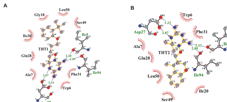
Fig 5. Interactions of (A) THT1 and (B) THT2 with binding pocket residues in DHFR. Residues in close contact and interacting through hydrophobic interactions are shown in red and H-bonds (green dots) and their distances are in green. Black lines depict residues forming polar contacts with the ligand.
