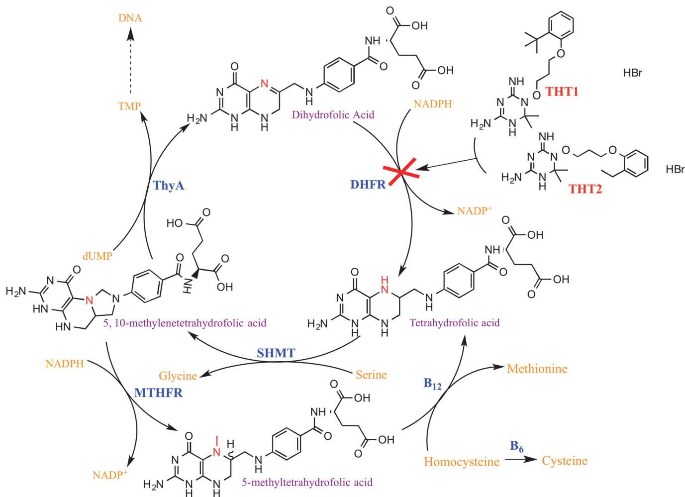
Fig 6. The biochemical relationship between ThyA and DHFR. Enzymes are highlighted in blue. ThyA, thymidylate synthase; DHFR, dihydrofolate reductase; SHMT, serine hydroxymethyltransferase; DHF, dihydrofolate; THF, tetrahydrofolate; mTHF, methyl tetrahydrofolate.
