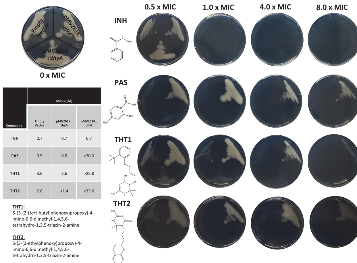
Fig 3. Impact on the MIC of THT1 and THT2 upon the over-expression of ThyA and DHFR with Isoniazid (INH) and para-aminosalicylic acid (PAS) as negative and positive controls. The MICs of THT1 and THT2 were determined in M. bovis BCG containing pMV261, pMV261::thyA and pMV261::dfrA. Plates are shown at 0.5, 1.0, 4.0 and 8.0 x MIC of each compound (with respect to the empty vector), the structures of which are given along with the IUPAC nomenclature for THT1 and THT2 and tabulated MIC data.
