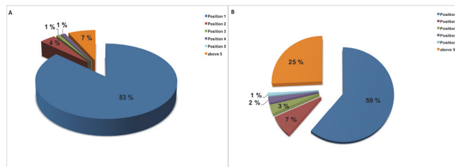
Fig 1. The multiple category naïve Bayesian classifier validation results. (A) Validation results of the model generated from randomly selected 80% target-ligand pairs and the remaining 20% was used as a test set. (B) Validation results of the model built using target-ligand pairs from 80% of the published articles and the test set consisted of target-ligand pairs from the remaining 20%.
