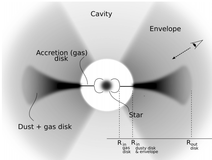
Fig. 4. Schematic picture of the model geometry of the object (not to scale). The line of sight crosses through the envelope. The inclination of the disk is \vartheta \approx 60^\circ , the opening angle of the conical cavity is 50^\circ (AP07).
