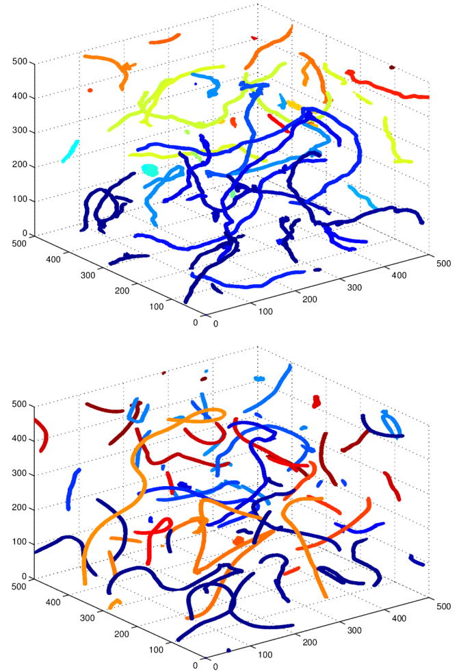
FIG. 2 (color online). Two snapshots of the simulations with \beta = 0.04 in radiation (top) and matter (bottom). The top figure shows that strings in the radiation era are fuzzier, and many of the segments have energy lumps attached to them. The bottom figure shows segments that are in general smoother—an obvious consequence of the additional damping (there is less radiation in the box). Note that in either snapshot only part of the simulated box is depicted.
