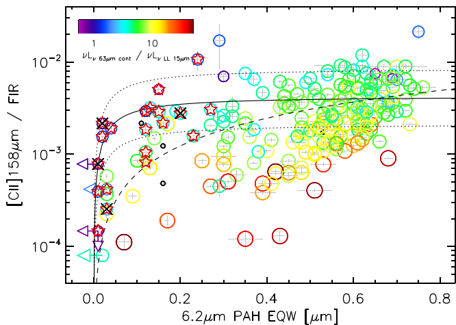
Figure 6. [\text{C II}]157.7 \mu\text{m}/\text{FIR} ratio for individual galaxies in the GOALS sample as a function of the 6.2 \mu\text{m} PAH EW measured with Spitzer /IRS. Galaxies are color-coded as a function of their \nu L_{\nu} 63/15 \mu\text{m} ratio. If this information is not available, galaxies are shown as small black circles. The solid line represents the range in [\text{C II}]/\text{FIR} and 6.2 \mu\text{m} PAH with increasing contribution from an AGN (see text for details). The dotted lines are \times 2 and \times 0.5 the predicted trend, which accounts for variations in the [\text{C II}]/6.2 \mu\text{m} PAH ratio and the L_{\text{FIR}}/\nu L_{\nu} 6 \mu\text{m} relation for star-forming galaxies. The dashed line assumes a decreasing of the [\text{C II}]/6.2 \mu\text{m} PAH ratio proportional to the 6.2 \mu\text{m} PAH EW due to pure PAH destruction from an AGN.
