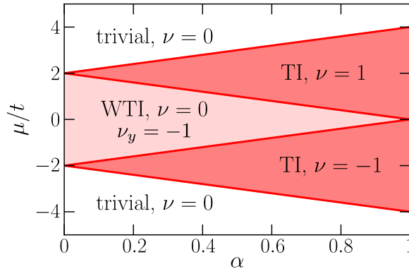
Figure 3. Phase diagram of the class-D Hamiltonian (3) in the absence of disorder ( \delta = 0 ), as a function of chemical potential \mu and anisotropy \alpha . The strong topological insulator phases (TI) have chiral Majorana modes along all edges, while the weak topological insulator phase (WTI) has Majorana modes only along edges oriented in the y -direction. The trivial phase has no edge modes.
