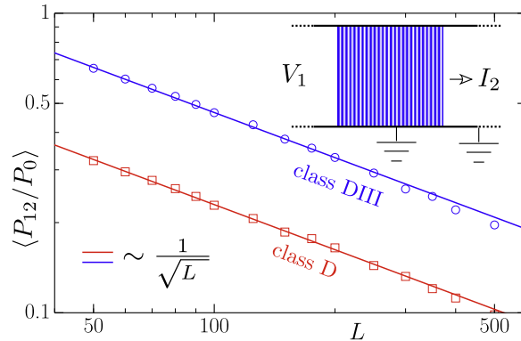
Figure 13. Disorder-averaged electrical shot noise power (23) in the WTI phase of class D and DIII, for parameters as in figure 11. Data points are averaged over 10^4 disorder realizations. The solid lines show that this electrical transport property obeys the same L^{-1/2} scaling as the thermal transport property of figure 11. The inset shows the geometry, with one metal contact biased at voltage V_1 and both the superconductor and the second metal contact grounded. The electrical current I_2 into this second contact fluctuates in time with noise power P_{12} = \int_{-\infty}^{\infty} dt \langle \delta I_2(0) \delta I_2(t) \rangle .
