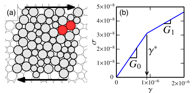
FIG. 1. (Color online) (a) The first contact change in a sheared packing ( N = 64 , P = 10^{-6} ) occurs at a strain \gamma^* = 9.003\,851(2) \times 10^{-7} , when the two marked particles lose their contact. (b) The corresponding stress-strain curve remains continuous but exhibits a sharp kink; we define G_0 as the shear modulus of the undeformed packing, and G_1 as the shear modulus of the packing just above \gamma^* .
