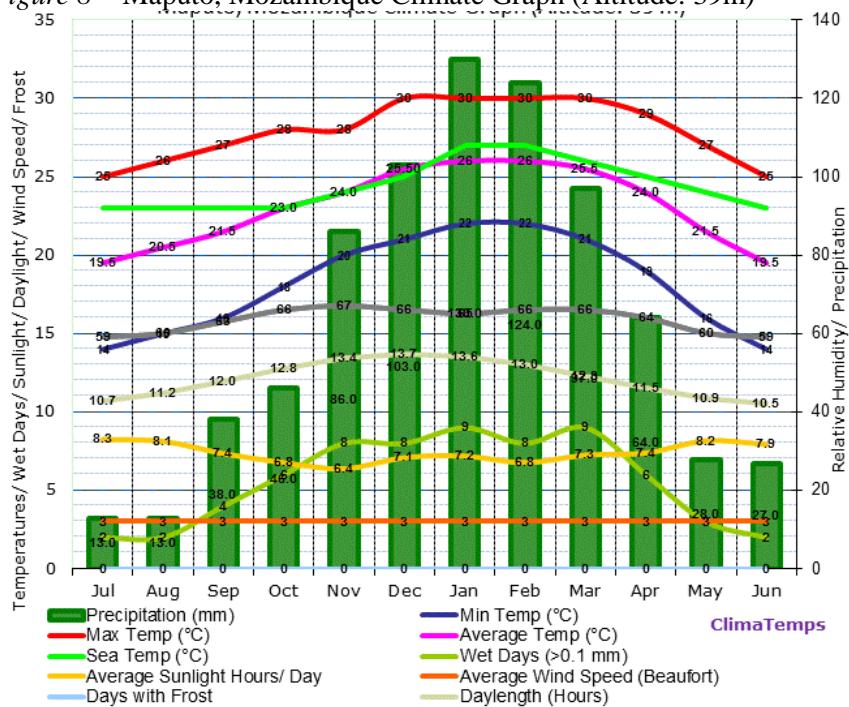
Figure 8 Maputo, Mozambique Climate Graph (Altitude: 39m)
