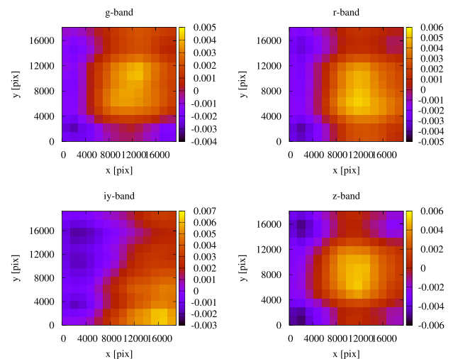
Figure 7. Distributions of magnitude differences of stars with respect to SDSS in pixel coordinates after photometric re-calibration. This reveals a pattern in the offset w.r.t. SDSS as a function of position in the CCD mosaic, which is likely caused by an imperfect scattered-light/illumination correction.
