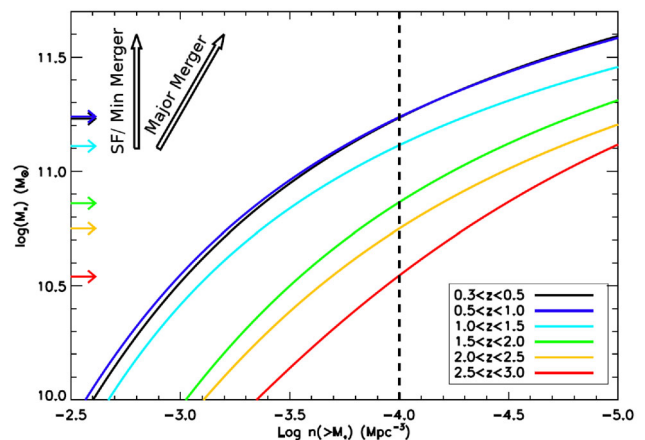
Figure 1. The integrated stellar mass functions from z = 0.3 to 3 from Mortlock et al. (2015). These integrated stellar mass functions give us the comoving number density of all galaxies more massive than at a given stellar mass. The large open black arrows indicate the expected evolution due to star formation, minor mergers, and major mergers. We compare galaxies at a constant number density by selecting galaxies at each redshift at limits of n(> M_*) = 10^{-4} \text{ Mpc}^{-3} . The black dashed vertical line denotes the constant number density of 10^{-4} \text{ Mpc}^{-3} . The coloured arrows indicate the values of M_* that correspond to this number density for each integrated stellar mass fraction.
