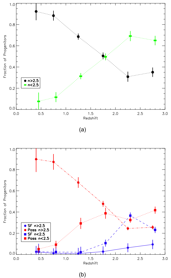
Figure 10. Fraction of the progenitors of local massive galaxies with high ( n > 2.5 ) and low ( n < 2.5 ) Sérsic indices. Figure (a) show the evolution of the whole progenitor sample with, green rectangles showing the fraction of progenitors with low Sérsic index and, black circles showing progenitors with high Sérsic light profiles as a function of redshift. Error bars are derived using Monte Carlo analysis. Figure (b) shows the high and low Sérsic populations split into star-forming and passive systems.
