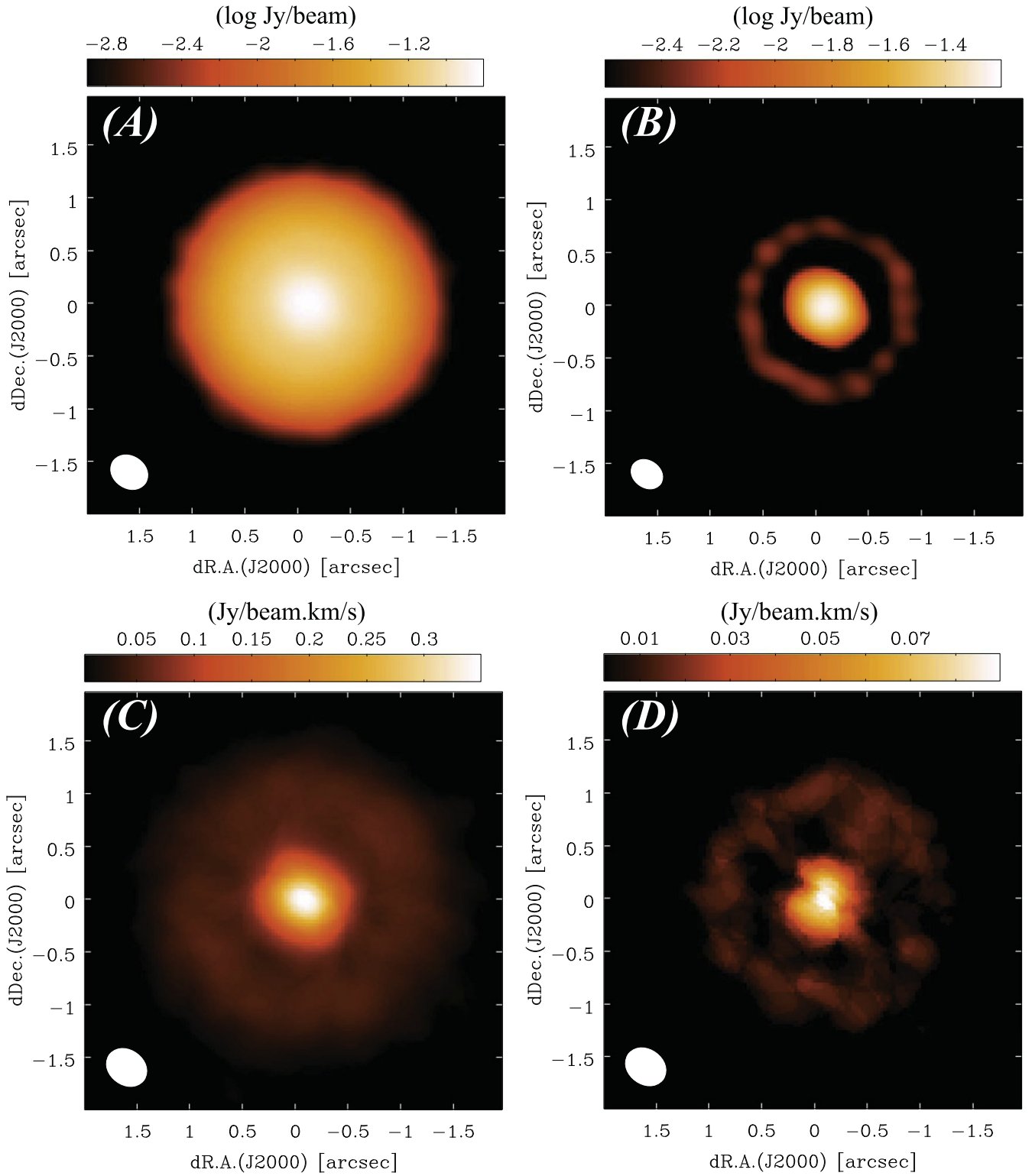
Figure 1. 336 GHz dust continuum map imaged using (A) all spatial frequency data, (B) only high spatial frequency ( >200\text{ k}\lambda ) data, and (C) ^{13}\text{CO } J=3-2 and (D) \text{C}^{18}\text{O } J=3-2 integrated line emission maps. Emission that was less than the 5\sigma noise level were masked. The synthesized beam sizes are shown in the bottom left corner of each panel.
