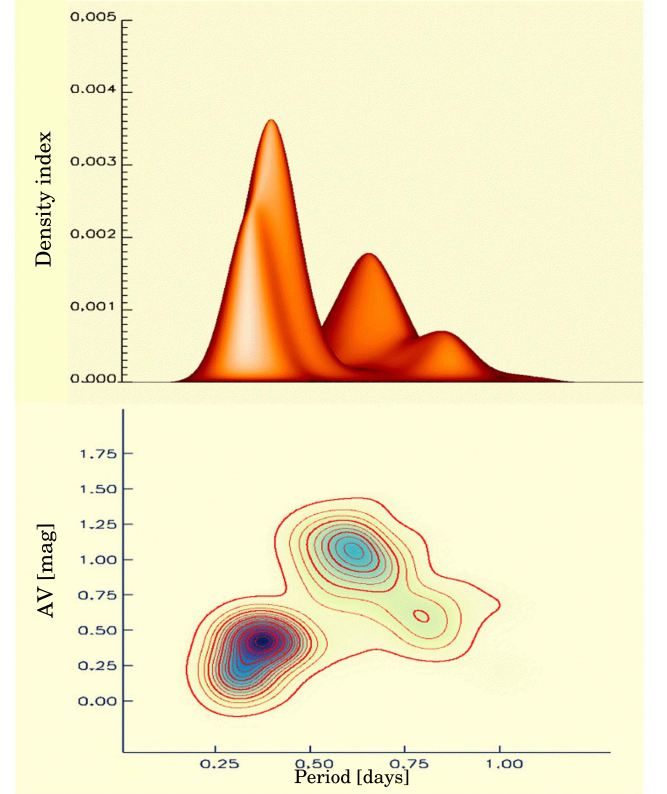
Figure 7. Top: 3D Bailey diagram for candidate \omega Cen RRLs: pulsation period in days, V -band amplitude and the Z -axis in arbitrary units. Bottom: same as the top, but with the view from the top.
