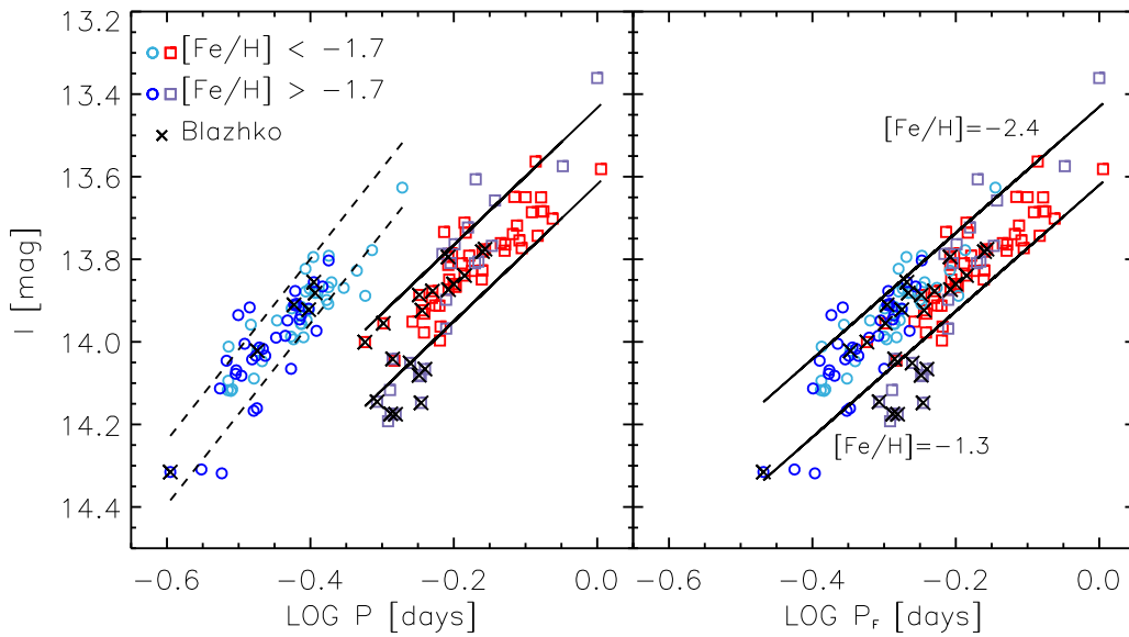
Figure 15. Left: empirical I -band PL relation for \omega Cen RRLs. Light blue circles and red squares mark variables more metal-poor than [\text{Fe}/\text{H}] = -1.7 , while blue circles and violet squares mark variables more metal-rich than [\text{Fe}/\text{H}] = -1.7 . Candidate Blazhko stars are marked with a black cross. The black lines display the predicted (Marconi et al. 2015) I -band PLZ relation for F (solid) and FO pulsators at fixed metal abundance [\text{Fe}/\text{H}] = -2.4 (brighter) and [\text{Fe}/\text{H}] = -1.3 (fainter). Right: same as left, but for the global (RRc+RRab) RRL sample. The periods of RRc variables were fundamentalized using \log P_{\text{RRab}} = \log P_{\text{RRc}} + 0.127 .
