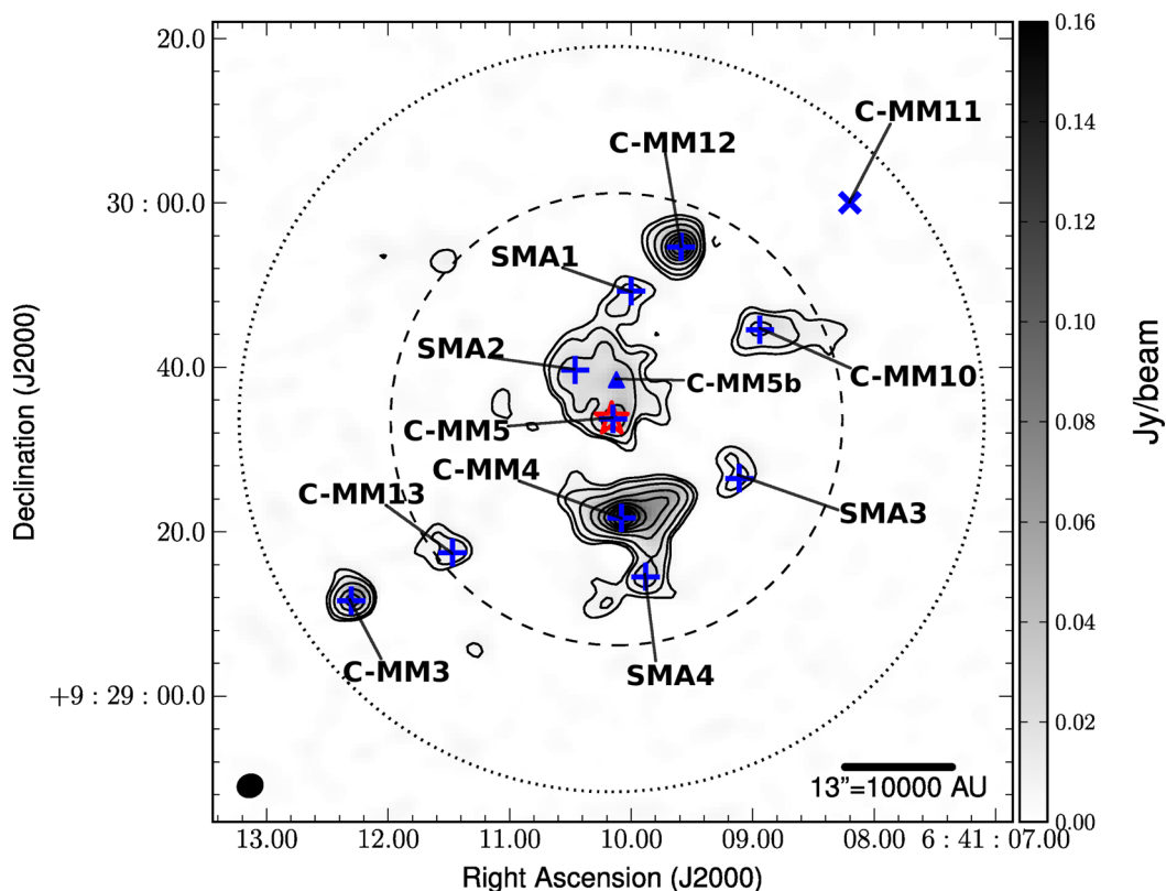
Figure 2. Map of the 1.3 mm continuum emission towards the section of NGC 2264-C observed with the SMA. The grey-scale shows the SMA 1.3 mm continuum emission from 0 to 0.16 Jy beam -1 ; the peak flux in the field is 0.159 Jy beam -1 . The black contours represent (3, 5, 10, 20, 30, 40, 50, 60, 70, 80) \times \sigma = 2 mJy beam -1 . The peak continuum positions for the 10 leaves (millimetre continuum peaks) identified in the dendrogram are marked with blue pluses (+) and labelled SMA – for new detections and C-MM – for previously detected sources. The blue triangle marks the peak position of the possible millimetre continuum peak C-MM5b. The red star represents the position of AFGL 989-IRS1, taken from the 2MASS data in the RMS survey, and the blue cross (x) marks the position of C-MM11 from Peretto et al. (2007). The black dashed circle represents the FWHP of the SMA primary beam, and the outer black dotted circle represents the 10 percent power level of the SMA primary beam. The SMA synthesized beam ( 3.06 \times 2.69 arcsec, PA = -69.3 ) is shown at lower left.
