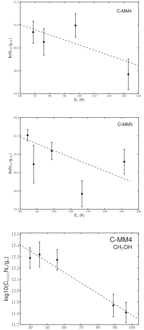
Figure 9. Rotation diagrams for \text{CH}_3\text{CN } J = 12_K - 11_K observed towards the continuum peaks of C-MM4 and C-MM5 (top two panels) and for \text{CH}_3\text{OH} towards the continuum peak of C-MM4 (bottom panel). The \text{CH}_3\text{OH} rotation diagram has been corrected for optical depth (Section 4.1.1).
