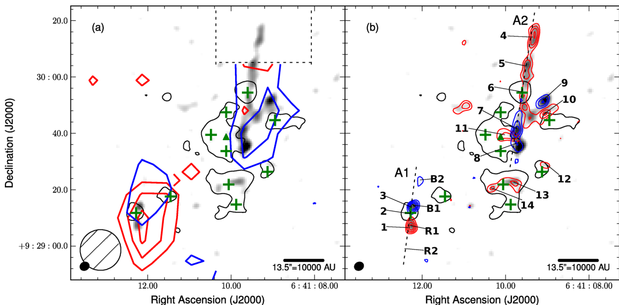
Figure 5. SiO kinematics. SMA SiO integrated intensity map (grey-scale, integrated over the velocity range -20 to 37 \text{ km s}^{-1} ) overlaid with contours of 1.3 \text{ mm} continuum emission (black contour, level 3\sigma = 6 \text{ mJy beam}^{-1} ) and blue/redshifted SiO emission from (a) the JCMT (SiO (8–7)) and (b) the SMA (SiO (5–4)). The velocity intervals for the blue/redshifted SiO begin 3 \text{ km s}^{-1} from the v_{\text{LSR}} ( v_{\text{LSR}} = 7.1 \text{ km s}^{-1} for C-MM3, 8.3 \text{ km s}^{-1} for C-MM4 and 8.9 \text{ km s}^{-1} for C-MM12, see Section 3.2.1) and extend to the maximum outflow velocity. The velocity intervals are the same for the JCMT and SMA data and are: blue: -20 to +4.1 \text{ km s}^{-1} for C-MM3 (and C-MM13), -1.0 to +5.3 \text{ km s}^{-1} for C-MM4, and -20 to +5.9 \text{ km s}^{-1} for C-MM12 (and the other millimetre continuum cores); red: +10.1 to +37 \text{ km s}^{-1} (C-MM3 and C-MM13), +11.3 to +20 \text{ km s}^{-1} (C-MM4), and +11.9 to +32 \text{ km s}^{-1} (C-MM12 and other cores). In both panels, green pluses (+) mark the positions of the 10 millimetre continuum peaks from the dendrogram analysis and the green triangle marks the position of C-MM5b. (a) JCMT SiO (8–7) contour levels: (3, 5, 7, 9) \times \sigma = 0.2 \text{ K km s}^{-1} . The 14.5 \text{ arcsec} JCMT beam (hatched circle) and the SMA synthesized beam (filled ellipse) are shown at lower left. The dashed rectangle shows the area of missing data from the HARP receiver element H14. (b) SMA SiO (5–4) contour levels: (3, 5, 7, 9) \times \sigma = 0.36 \text{ Jy beam}^{-1} \text{ km s}^{-1} . The dashed black lines represent the possible outflow axes A1 and A2. The numbered positions 1–14 mark the components discussed in Section 3.2.2, and mark the positions at which the spectra shown in Fig. 7 were extracted. Positions 1–3 are part of the outflow axis A1, positions 4–8 are part of outflow axis A2, and the remaining positions mark locations of ambiguous SiO emission that is not obviously associated with an outflow. The labels R1, R2, B1, and B2 mark the components of the redshifted and blueshifted outflow lobes of C-MM3 named by Saruwatari et al. (2011).
