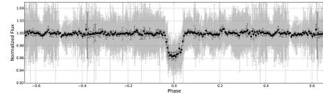
FIG. 1.— The phase-folded light curve. Black points denote data binned to 10 minutes in phase, while the gray points show the original data. Vertical lines show the uncertainties for single measurements.
