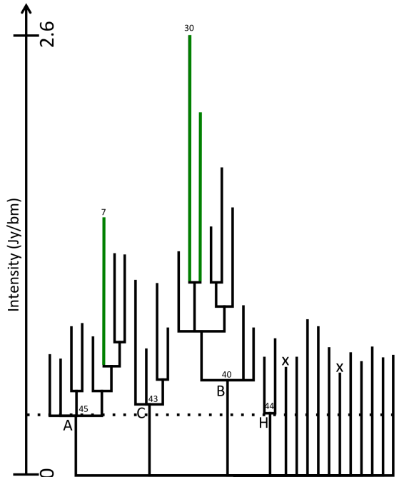
Fig. 8.— Same as Figure 7, but for the HCN non-binary dendrogram.
