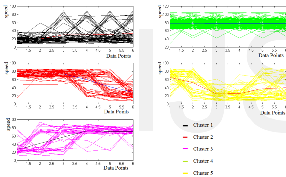
Fig. 5: K-means Clusters
