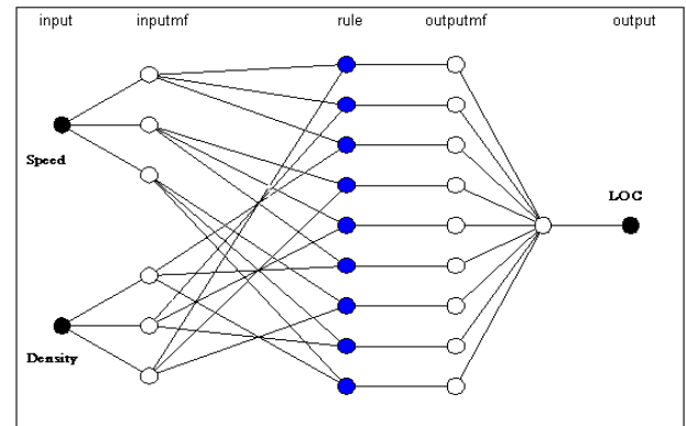
Fig. 3 Neuro-Fuzzy Model
