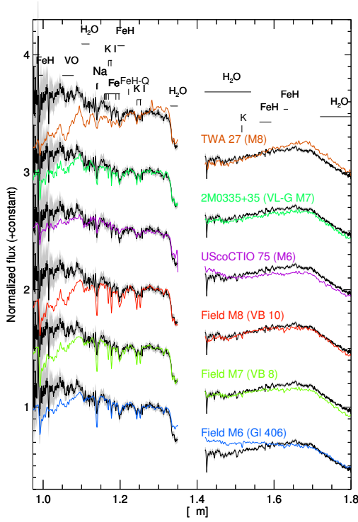
Fig. 11. Comparison of the MRS spectrum of PZ Tel B to those of field M6–M8 dwarfs.
