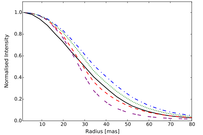
Fig. 7. Observed azimuthally-averaged radial profile of the total intensity in the second-epoch \text{cntH}\alpha images (full black line) compared to models with \tau_V = 0.65 , R_o = 1.5 R_\star , and n = 4 (dashed red line), \tau_V = 1.3 , R_o = 1.45 R_\star , and n = 4.5 (dotted green line), and \tau_V = 1.9 , R_o = 1.4 R_\star , and n = 5 (dotted-dashed blue line). The values of R_o and n for each of the dust models shown have been determined by fitting the radial profile of the polarised intensity. For reference, we also show the radial profile of our model star with no dust envelope (double-dashed purple line).
