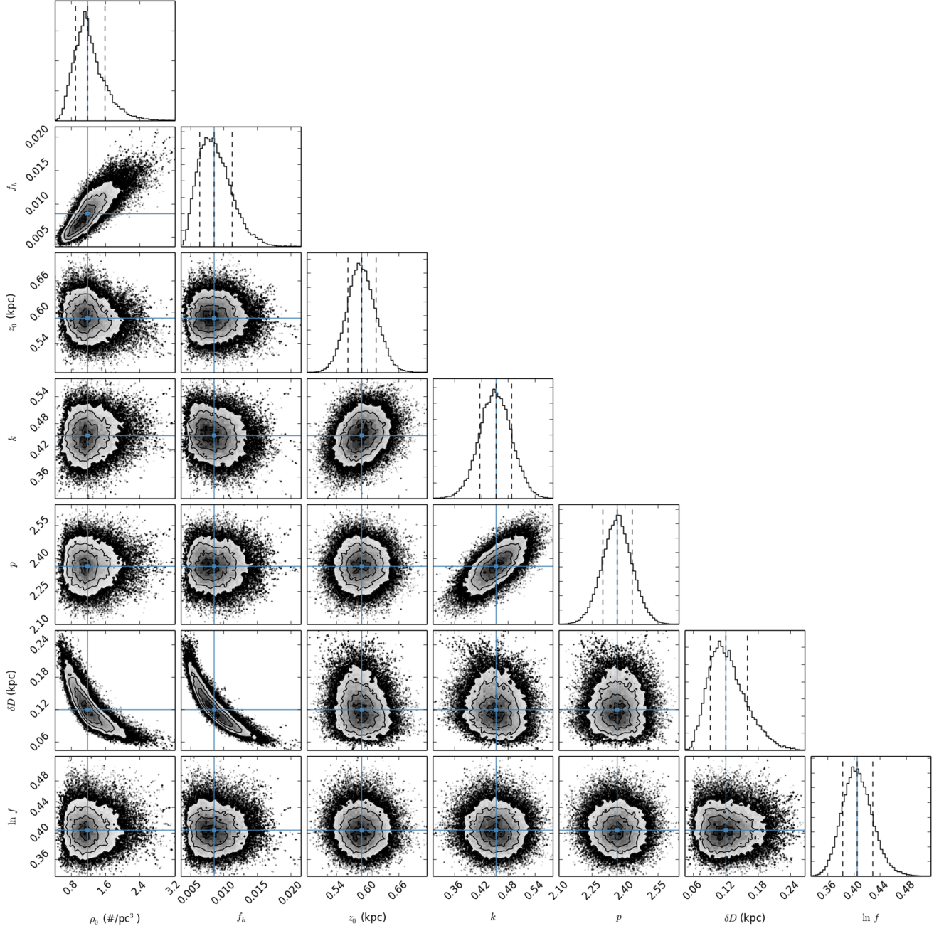
Figure 6. Halo–disc model ( h = 2.6 kpc): corner plot made with the scalength as a fixed parameter for subtypes M0 to M9. \rho_0 – \delta D and f_h – \delta D are degenerate. \rho_0 – f_h and \kappa – p show some degeneracy.
