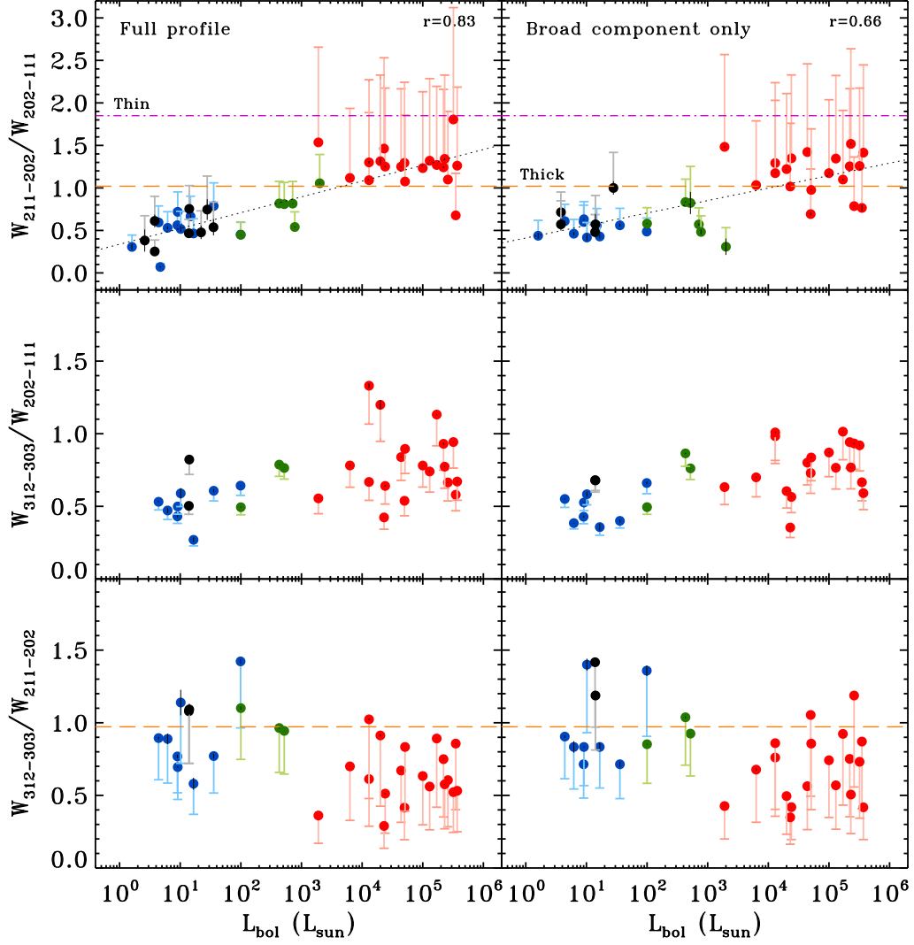
Fig. 4. ( Top panels ) Ratio of the integrated intensities of the 2_{11}-2_{02} (752 GHz) and 2_{02}-1_{11} (988 GHz) water lines versus the bolometric luminosity of the source. ( Middle panels ) Ratio of the integrated intensities of the \text{H}_2\text{O} 3_{12}-3_{03} (1097 GHz) and 2_{02}-1_{11} (988 GHz) spectra versus L_{\text{bol}} . ( Bottom panels ) Ratio of the integrated intensities of the 3_{12}-3_{03} (1097 GHz) and 2_{11}-2_{02} (752 GHz) water emission lines as a function of L_{\text{bol}} . The left-column presents the ratios calculated considering the entire line profile and the right-column shows the ratio of the integrated intensity calculated for the broad velocity component. The value of the ratios with and without correcting by the different beam size factors are indicated by dashed lighter lines and darker dot symbols respectively. Blue lines and symbols correspond to the low-mass Class 0 protostars, black to the low-mass Class I, green to intermediate-mass objects and red lines and symbols to high-mass YSOs. The purple dashed-dotted horizontal lines and the orange dashed horizontal lines indicate the optically thin and optically thick limits, respectively, calculated assuming LTE and an excitation temperature of 300 K. The linear correlation between the dot symbols (ratios not beam corrected) and the logarithm of the luminosity is shown by the dotted black lines in the top panels .
