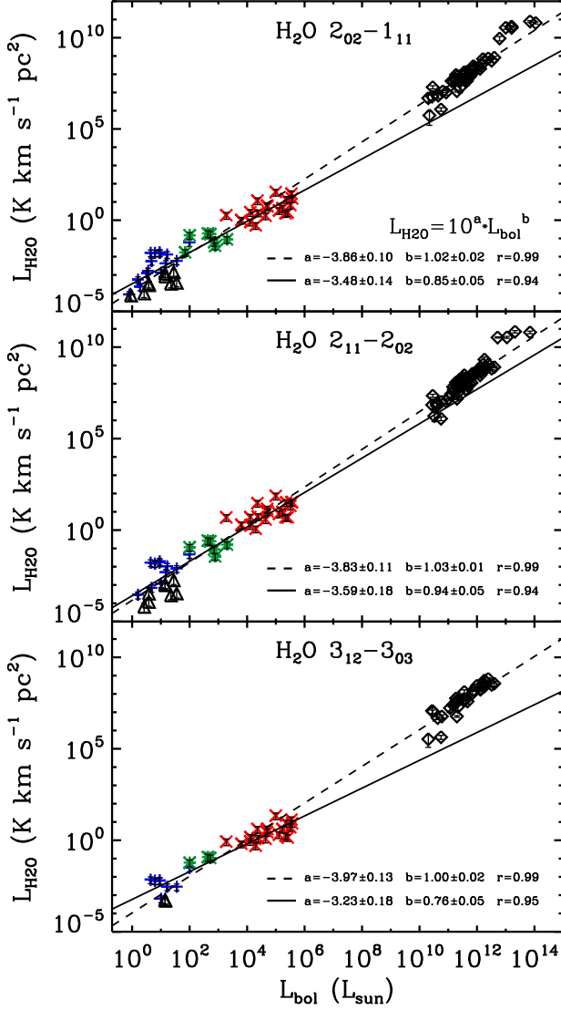
Fig. 9. Same as Fig.3 but including the line luminosity observed for several extragalactic sources (black diamonds) taken from Yang et al. (2013). The solid black line corresponds to the fit of the WISH YSOs and the dashed black line indicates the correlation including the values of extragalactic sources.
