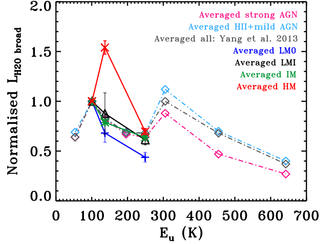
Fig. 10. Line luminosity of the water transitions normalised to the luminosity of the H 2 O 2 02 -1 11 (988 GHz) line as a function of the upper energy level ( E_u ) of each transition considering only the contribution from the cavity shock component. The solid blue, black, green and red lines corresponds to the averaged value of the normalised intensity for the low-mass Class 0, Class I, intermediate-mass and high-mass YSOs respectively. The grey dashed line represents the average values of the sample presented in Yang et al. (2013), the pink and light blue dashed lines indicate the values of the strong AGN- and HII+mild-AGN-dominated galaxies, respectively. The 2 11 -2 02 (752 GHz) line has an E_u/k_B = 137 K and the 3 12 -3 03 (1097 GHz) an E_u/k_B = 249 K.
