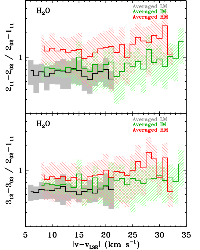
Fig. 5. Averaged H 2 O 2 11 -2 02 / 2 02 -1 11 ratio (top panel) and H 2 O 3 12 -3 03 /2 02 -1 11 line intensity ratio (bottom panel) as a function of offset velocity for the low-mass protostars (LM; grey area from Mottram et al. 2014), intermediate-mass objects (IM; green line and asterisks), and the high-mass YSOs (HM; red line and crosses). The dashed green and red regions indicate the calculated standard deviation of the line ratio for each velocity channel.
