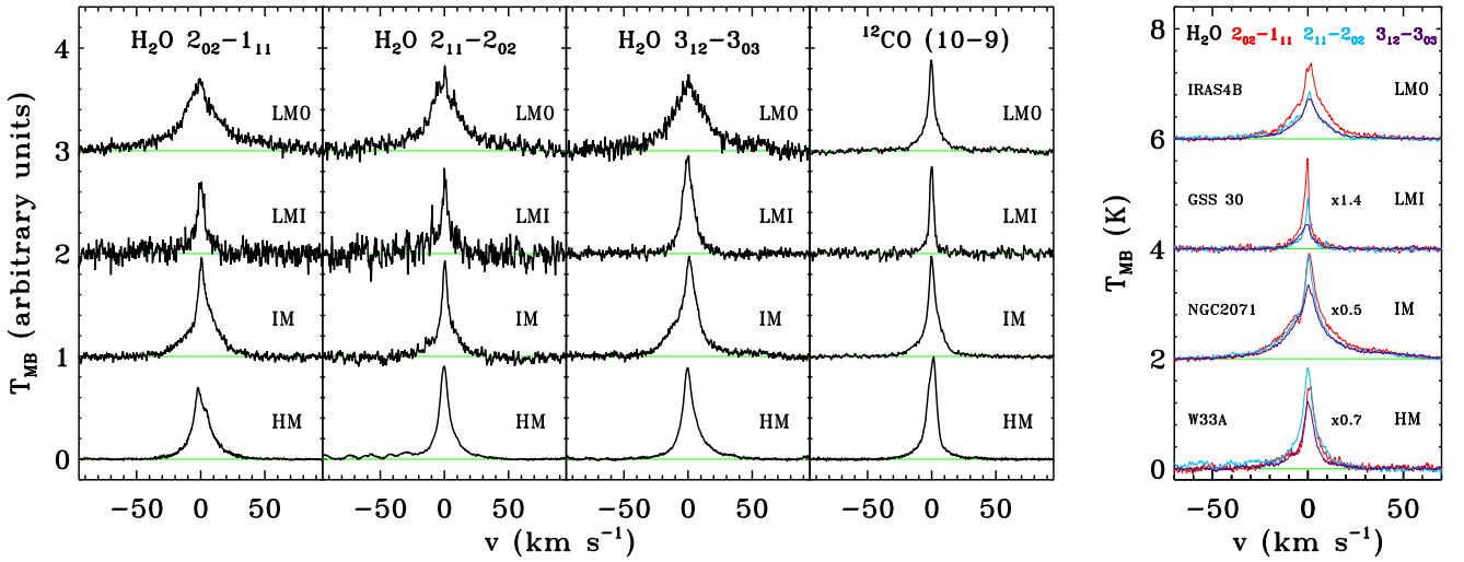
Fig. 1. Left figure: Averaged and normalised spectrum calculated for the low-mass Class 0 (LM0) protostars, the low-mass Class I (LMI), intermediate-mass YSOs (IM) and high-mass objects (HM) for the H 2 O 2 02 -1 11 988 GHz (left panel), 2 11 -2 02 752 GHz (middle-left panel), 3 12 -3 03 1097 GHz (middle-right panel) transitions and the 12 CO J =10–9 (right panel) spectra (see San José-García et al. 2013). The spectra of each sub-group of YSOs have been shifted vertically for visualisation purposes. The low intensity features on the blue wing of the H 2 O 2 11 -2 02 high-mass profile are due to methanol emission. Right figure: H 2 O 2 02 -1 11 , 2 11 -2 02 and 3 12 -3 03 spectra plotted in red, blue and purple respectively for NGC 1333 IRAS4B (LM0), GSS 30 (LMI), NGC2071 (IM) and W33A (HM). The horizontal light green lines in both figures represent the baseline level.
