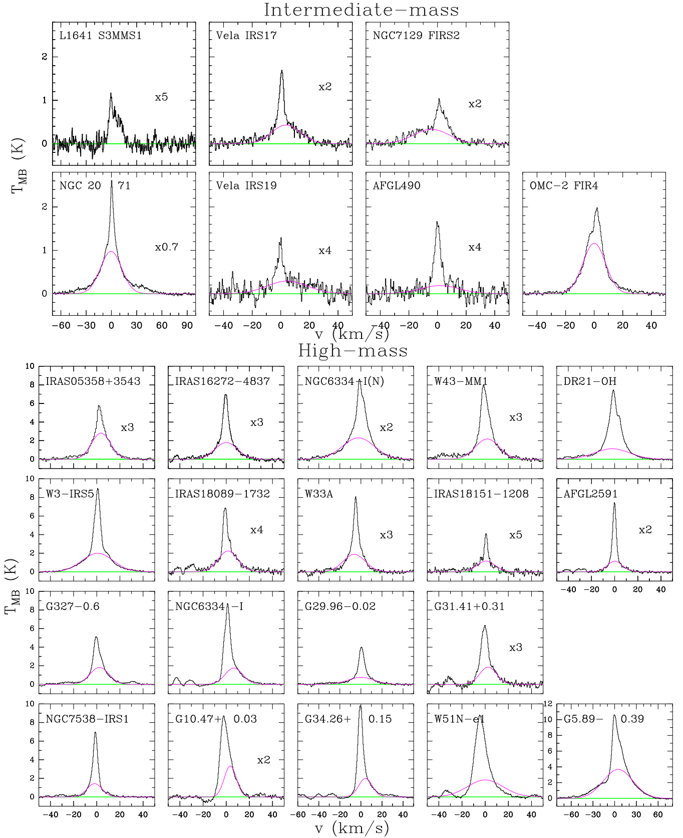
Fig. A.2. \text{H}_2\text{O} 2_{11}-2_{02} spectra for the intermediate-mass YSOs ( top ) and high-mass sources ( bottom ). The green line represents the baseline level and the pink Gaussian the broad velocity component. All spectra have been shifted to zero velocity. The numbers indicate where the spectra have been scaled for greater visibility.
