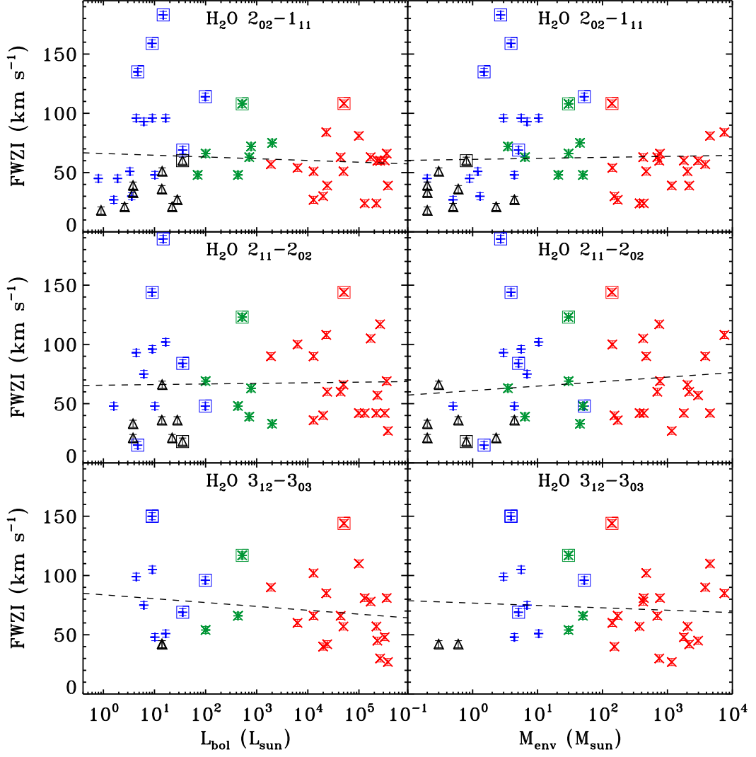
Fig. C.2. ( Left-column ) FWZI of the H 2 O 2 02 -1 11 988 GHz ( top panel ), 2 11 -2 02 752 GHz ( middle panel ) and 3 12 -3 03 1097 GHz ( bottom panel ) transitions as a function of the bolometric luminosity of each source. ( Right-column ) Same as left-column but versus the envelope mass of each YSO. The blue plus symbols correspond to the low-mass Class 0 protostars, the black triangles the low-mass Class I, the green asterisks to the intermediate-mass objects and the red crosses to the high-mass YSOs. The low- and intermediate-mass objects with detected EHV components are surrounded by a box, as well as the high-mass YSO with triangular line profiles. FWZI is calculated by binning the spectra to 3 km s -1 .
