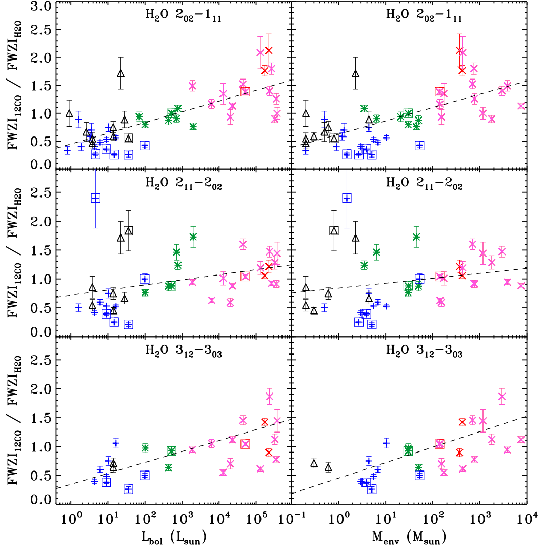
Fig. C.3. ( Left-column ) Ratio of the FWZI of the H 2 O 2_{02}-1_{11} 988 GHz ( top panel ), 2_{11}-2_{02} 752 GHz ( middle panel ) and 3_{12}-3_{03} 1097 GHz ( bottom panel ) transitions and the FWZI of the 12 CO observations as a function of the bolometric luminosity. ( Right-column ) Same as left-column but versus the envelope mass of each YSO. The low- and intermediate-mass sources with detected EHV components are surrounded by a box, and also the high-mass YSO with triangular line profiles. Both values of FWZI were calculated by binning the spectra to 3 km s -1 . The symbol and colour code is the same as in Fig. 2.
