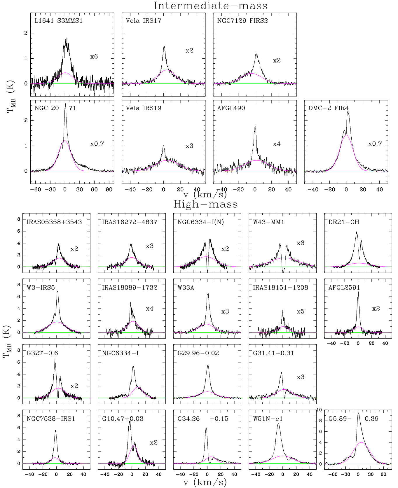
Fig. A.1. \text{H}_2\text{O } 2_{02-1_{11}} spectra for the intermediate-mass YSOs ( top ) and high-mass sources ( bottom ). The green line represents the baseline level and the pink Gaussian the broad velocity component. All spectra have been shifted to zero velocity. The numbers indicate where the spectra have been scaled for greater visibility.
