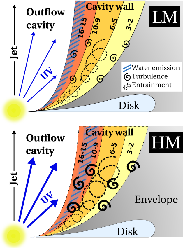
Fig. 8. Cartoon illustrating a scenario with a simplified physical structure of the different layers composing the outflow cavity wall for a representative low-mass protostar (LM; top panel) and for a high-mass YSO (HM; bottom panel). The emitting area of the low- J ^{12}\text{CO} transitions is shaded in yellow, that of the mid- J transitions is orange and of the high- J lines in red. Turbulent motions are represented with spiral symbols, the entrained material with swirls and the excited water emission is indicated with blue lines over the red region.
