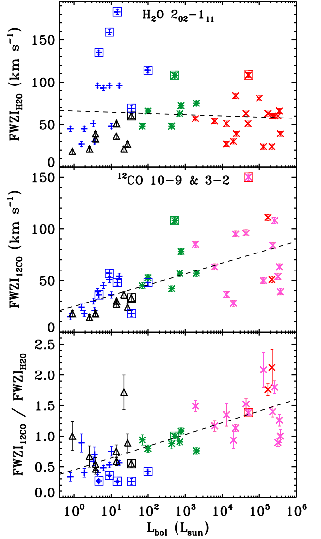
Fig. 2. (Top) FWZI of the \text{H}_2\text{O } 2_{02}-1_{11} (988 GHz) emission line versus the bolometric luminosity. (Middle) Same as top panel but for the ^{12}\text{CO } J=10-9 and J=3-2 observations. (Bottom) Ratio of the ^{12}\text{CO} and \text{H}_2\text{O } 2_{02}-1_{11} FWZI values as a function of L_{\text{bol}} . The blue plus symbols correspond to the low-mass Class 0 protostars, the black triangles the low-mass Class I, the green asterisks the intermediate-mass objects, the pink crosses the high-mass YSOs for which the ^{12}\text{CO } J=3-2 spectra are used, and the red cross symbols the high-mass object for which ^{12}\text{CO } J=10-9 data are available (see San José-García et al. 2013). The low- and intermediate-mass sources with detected EHV components are surrounded by a box, as well as the high-mass YSO with triangular water line profiles.
