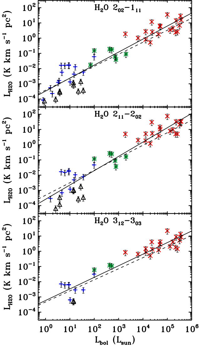
Fig. 3. Line luminosity of the H 2 O 2 02 -1 11 (988 GHz) line emission ( top ), the H 2 O 2 11 -2 02 (752 GHz) data ( middle ), and H 2 O 3 12 -3 03 (1097 GHz) spectra ( bottom ) versus the bolometric luminosity of the source. The blue pluses correspond to the low-mass Class 0 protostars, the black triangles the low-mass Class I, the green asterisks the intermediate-mass objects and the red cross symbols the high-mass YSOs. The solid line indicates the linear correlation of the logarithm of the total line luminosity, \log(L_{\text{H}_2\text{O}}) , and \log(L_{\text{bol}}) . The dashed line shows the log-log correlation of the luminosity measured for the broader Gaussian velocity component only (cavity shock emission; L_{\text{broad H}_2\text{O}} ) and \log(L_{\text{bol}}) .
