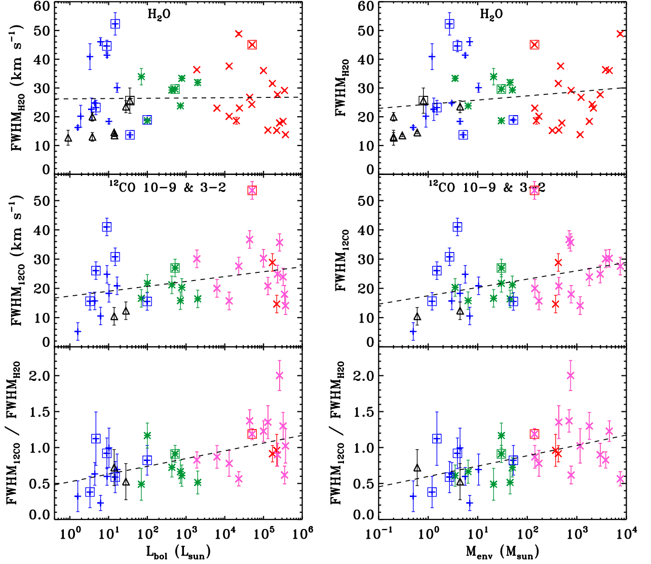
Fig. C.1. ( Left-column figure ) Derived \text{FWHM}_b of the Gaussian profile fitted to the cavity shock component of the \text{H}_2\text{O} lines ( top-panel ) as a function of bolometric luminosity. Constrained \text{FWHM}_b for the ^{12}\text{CO} J=10-9 and J=3-2 observations ( middle-panel ) versus L_{\text{bol}} . Ratio calculated from the ^{12}\text{CO} \text{FWHM}_b divided by the \text{FWHM}_b of the \text{H}_2\text{O} lines ( bottom-panel ) as a function of L_{\text{bol}} . ( Right-column figure ) Same as left- figure but plotted versus the envelope mass of the source, M_{\text{env}} . The blue plus symbols correspond to the low-mass Class 0 protostars, the black triangles the low-mass Class I, the green asterisks the intermediate-mass objects, the pink crosses the high-mass YSOs for which the ^{12}\text{CO} J = 3-2 spectra are taken, and the red cross symbols the high-mass object for which ^{12}\text{CO} J = 10-9 data are available (see San José-García et al. 2013). The low- and intermediate-mass objects with detected EHV components are surrounded by a box. Also the high-mass YSO with triangular water line profiles is surrounded by a box. The value of the \text{FWHM}_b of the different velocity components is calculated as explained in Sect. 2.5 and these parameters are the same for the three water transitions.
