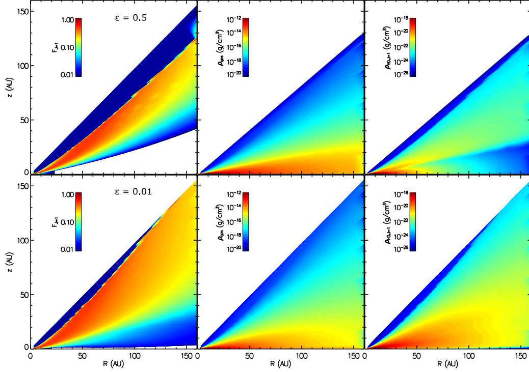
FIG. 7.— DM Tau disk structures. Upper row : fractional HD population in the J=1 level (left), gas density structure (center), and HD J=1 density structure (right) for \epsilon_{small}=0.5 (50% less dust). Lower row : fractional HD population in the J=1 level (left), gas density structure (center), and HD J=1 density structure (right) for \epsilon_{small}=0.01 (99% less dust).
