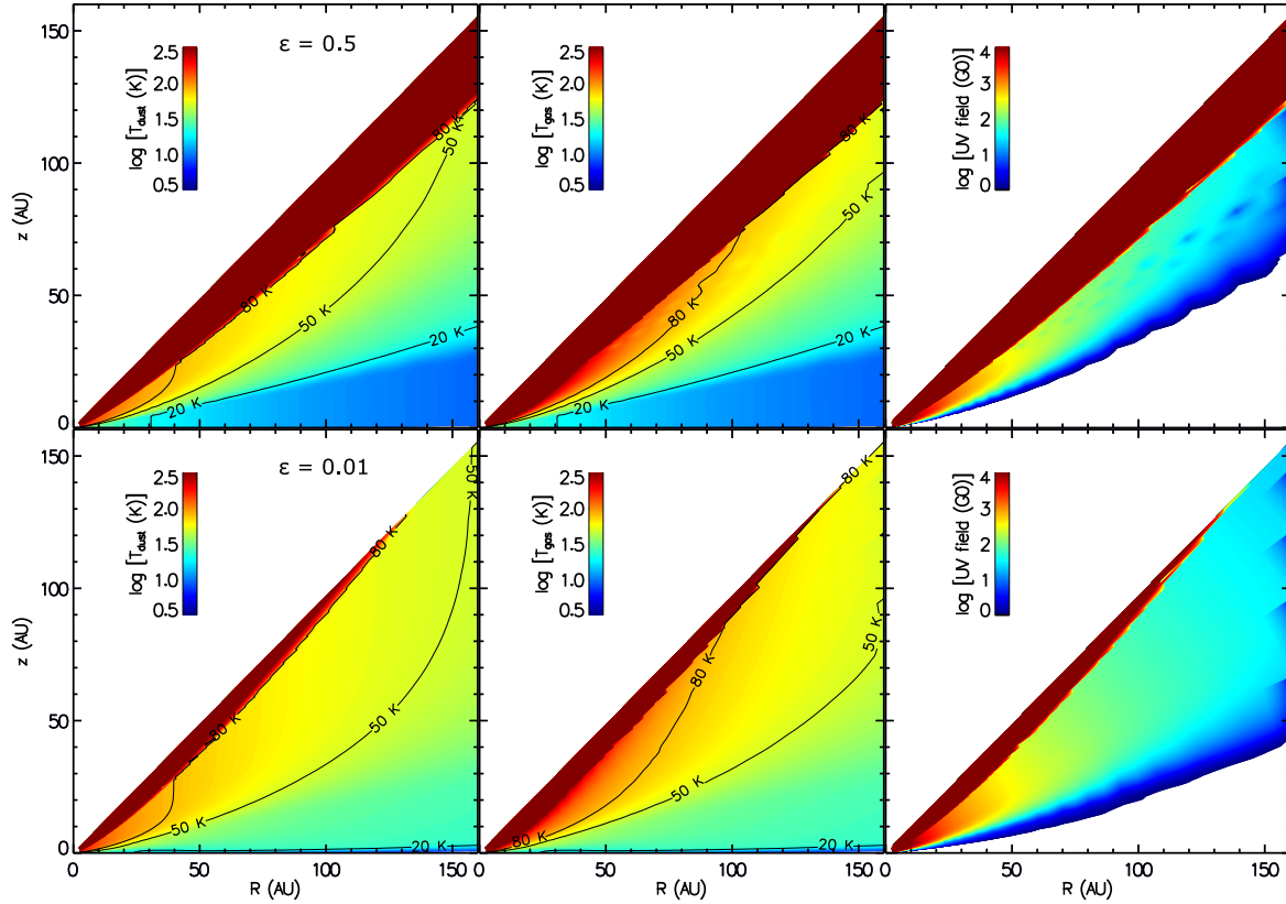
FIG. 4.— DM Tau disk structures. Upper row : dust and gas temperature and UV flux structures for \epsilon_{\text{small}}=0.5 (50% less dust). Lower row : dust and gas temperature and UV flux structures for \epsilon_{\text{small}}=0.01 (99% less dust). The UV radiation field is given in units of G0, or 1 Habing unit, equal to 1.6 \times 10^{-3} \text{ erg s}^{-1} \text{ cm}^{-2} .
