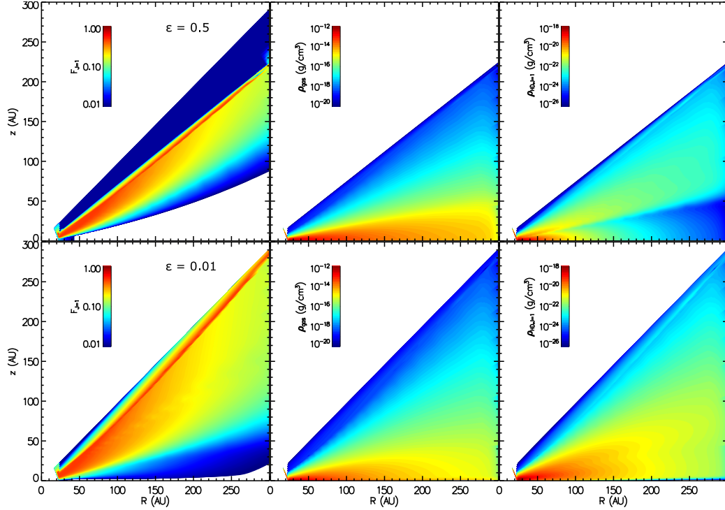
FIG. 8.— GM Aur disk structures. Upper row : fractional HD population in the J=1 level (left), gas density structure (center), and HD J=1 density structure (right) for \epsilon_{small}=0.5 (50% less dust). Lower row : fractional HD population in the J=1 level (left), gas density structure (center), and HD J=1 density structure (right) for \epsilon_{small}=0.01 (99% less dust).
