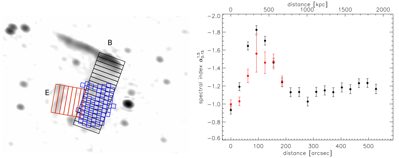
Figure 8. Left: regions where spectral indices were extracted are shown on top of the VLA 1–2 GHz image. The spectral indices for the red and black regions are shown in the left right panel. The spectra for the blue regions are shown in Figure 16. We excluded the regions affected by a compact source located at R.A. 06^{\text{h}}03^{\text{m}}23^{\text{s}} , Decl. 42^{\circ}13'26'' . Right: the spectral index between 0.15 and 1.5 GHz across the E radio relic is shown in red (from east to west). The spectral index across relic B1 and the radio halo, from north to south, is shown in black. The regions have a width of 31'' .
