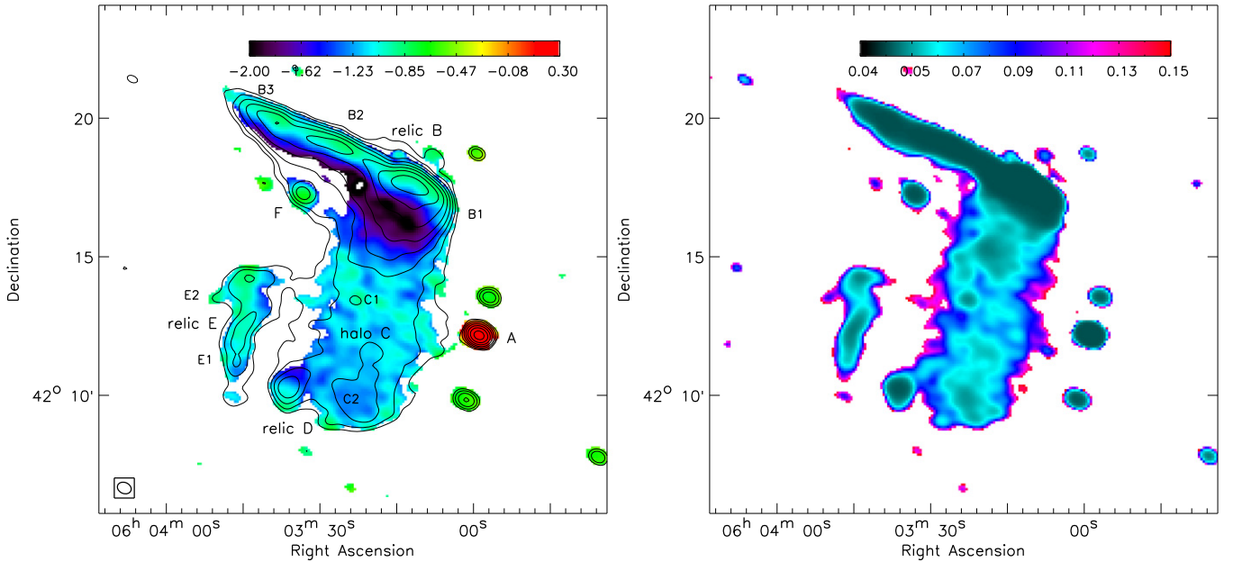
Figure 7. Left: spectral index map between 0.151 and 1.5 GHz at 31'' \times 24'' resolution. Sources are labelled as in Figure 1). Black contours are drawn at levels of [1, 2, 4, \dots] \times 2 \text{ mJy beam}^{-1} and are from the 0.151 GHz image. Pixels with values below 3.5\sigma_{\text{rms}} were blanked. Right: corresponding spectral index error map. The errors are based on the individual rms noise levels in the two maps and using an absolute flux calibration uncertainty of 10% at 150 MHz and 2.5% at 1.5 GHz.
