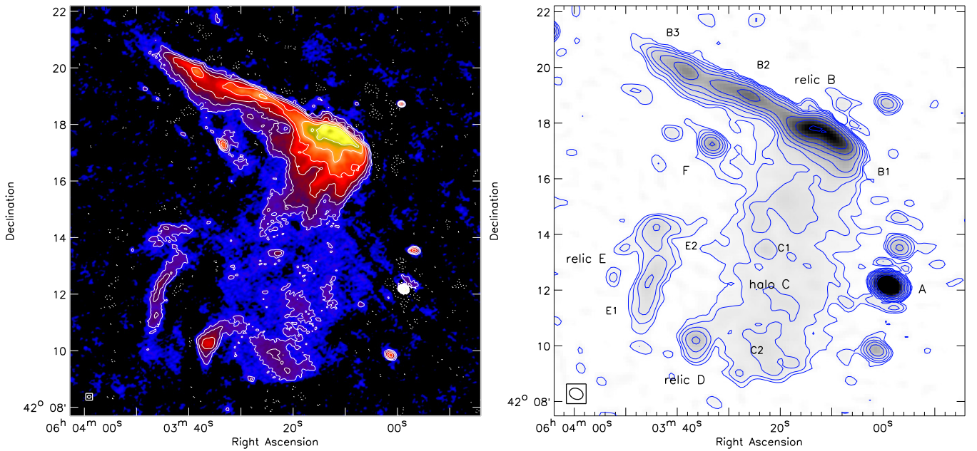
Figure 1. Left: LOFAR HBA 120–181 MHz image. The beam size is 8'' \times 6'' as indicated in the bottom left corner. Contour levels are drawn at [1, 2, 4, 8, \dots] \times 4\sigma_{\text{rms}} , with \sigma_{\text{rms}} = 93 \mu\text{Jy beam}^{-1} . Negative -3\sigma_{\text{rms}} contours are shown with dotted lines. Right: D-array VLA 1–2 GHz image with various sources labelled, following van Weeren et al. (2012a). Some of the sources are further subdivided into numbered components, e.g., relic E is divided into E1 and E2. The beam size is 31'' \times 24'' . Contour levels are drawn at the same levels as in the left panel, but with \sigma_{\text{rms}} = 35 \mu\text{Jy beam}^{-1} .
