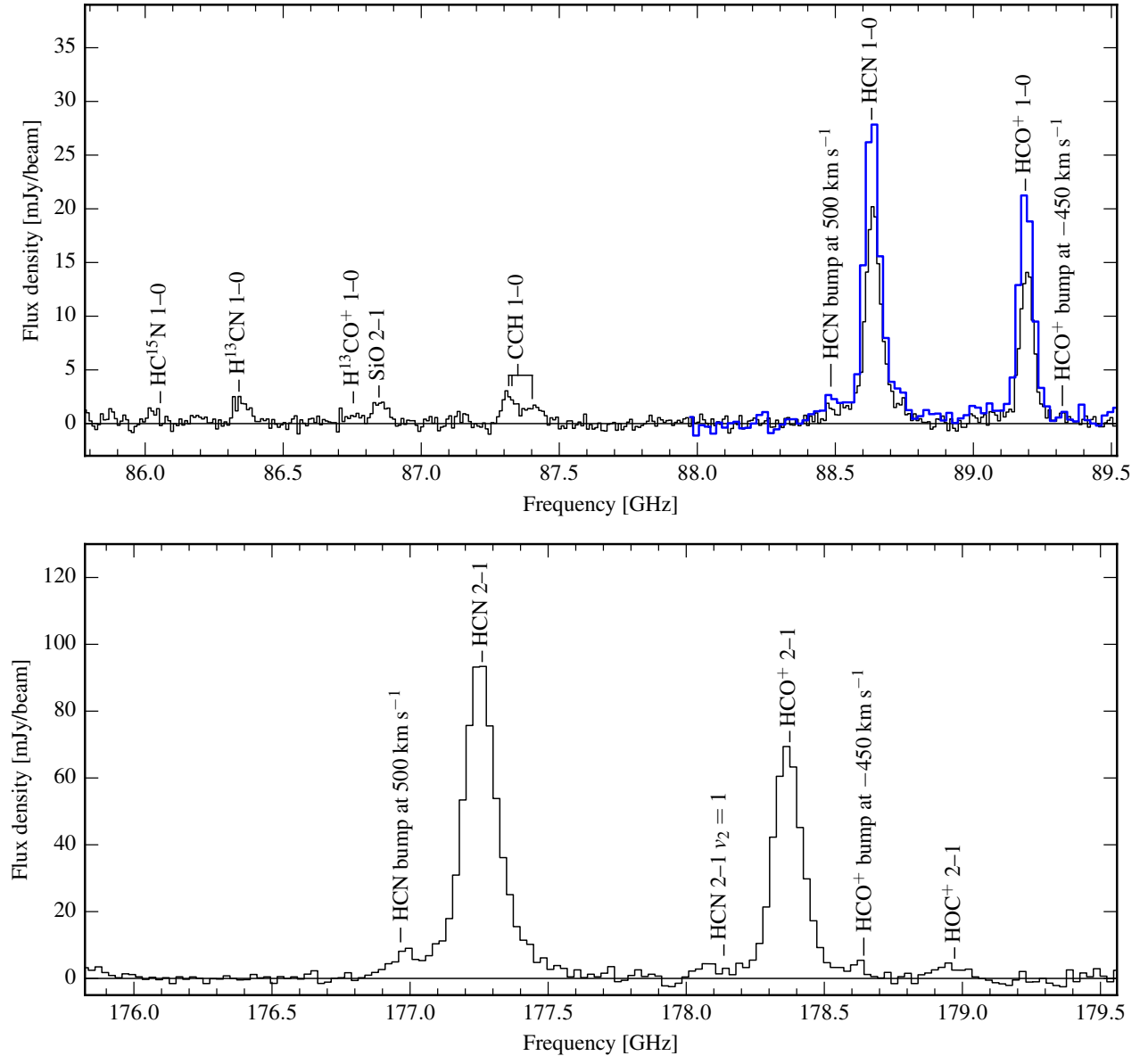
Fig. 1. Top: 3 mm A-array (black line) and B-array (thick blue line; Aalto et al. 2012a) spectra of Mrk 231 towards the central beam. Bottom: 2 mm D-array spectrum. The frequency of the HCN 2–1 \nu_2 = 1 line is indicated in the plot, but this line is not significantly detected. Both figures: the most prominent outflow bumps of HCN and HCO + emission are also indicated. The frequency axes of the two spectra are corrected for the redshift of the source ( z = 0.042170 ). The beam sizes can be found in Table 1.
