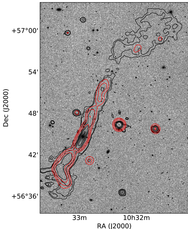
Figure 21. The giant radio galaxy HB13. The grey-scale image shows the optical image from DSS overlaid with NVSS 1.4-GHz contours in red (1, 2.5 and 5 \text{mJy beam}^{-1} ) and LOFAR 150-MHz contours in black (0.75, 1, 2.5, 5 and 10 \text{mJy beam}^{-1} ).
