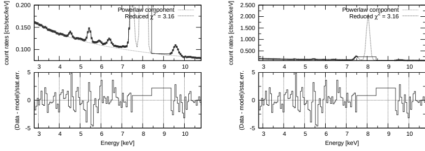
(a) The same as in Fig. 5.18 but now the relative contribution of primary gaussian, continuum and secondary gaussian is not fixed and determined from the least-squares method. (b) The same as is Fig. 5.19a but scaled for better visualization of high-energy line.
