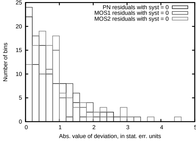
Figure 5.23: Distribution of residuals for MOS (Fig. 5.22, upper panels) and PN (Fig. 5.21, upper panel) cameras in the final dataset. The distribution is slightly non-Gaussian, especially due to presence of several large residuals. By adding a systematic error (0.19% for MOS1, 0.41% for MOS2 and 0.21% for PN camera) in quadratures we increase total error so the distribution (in units of total errors) becomes close to Gaussian, see Sec. 5.3.5 for calculation details.
