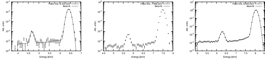
(a) Shape of strong instrumental line at 6.420 keV.
