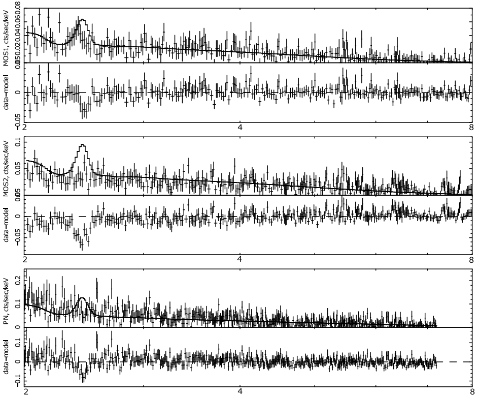
Figure 4.4: The spectra of off-center M31 observation 0402560301 (M31off, Sec.4.1.3.3). The decaying dark matter signal, obtained by proper scaling of the result of [316] is also shown. The error bars include 5% of the model flux as an additional systematic error. Fitting these spectra together excludes the properly scaled line of [316], at the level of at least 10.4\sigma (see text).
