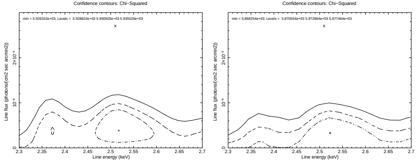
Figure 4.7: Left: \Delta\chi^2 = 2.3 (dashed-dotted), 4.61 (dashed) and 9.21 (solid) contours (corresponding to 68%, 90% and 99% confidence intervals) for a thin gaussian line allowed by the joint fit of M31out spectra used in this work. The resulting line normalizations are shown for an averaged dark matter column density in the M31out region (about 170M_{\odot}\text{pc}^{-2} , including the Milky Way contribution). The rescaled [316] line is marked with a cross x; its normalization is therefore 4.50 \times 10^{-8} \times \frac{170}{208.5+73.9} = 2.71 \times 10^{-8}\text{photons cm}^{-2}\text{sec arcmin}^{-2} . It is clearly seen that the hypothesis of dark matter origin for a [316] line-like feature is excluded at extremely high significance, corresponding to more than \approx 10\sigma (see text). Right: The same as in the left figure but with an addition of a bknpow/b component to model the contribution of the remaining soft proton contamination (see text). The break energy is fixed as 3.2 keV so no degeneracy with the parameters of the gaussian is expected. The bknpow/b powerlaw indices at low and high energies are fixed to be the same for different cameras observing the same spatial region. The line significance drops below 1\sigma in this case.
