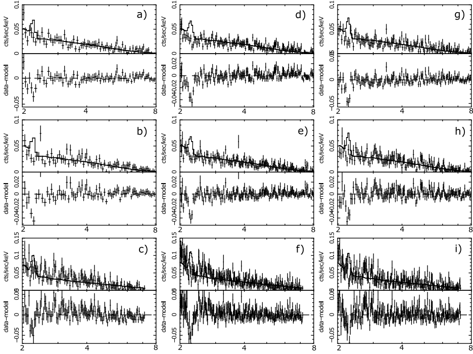
Figure 4.3: Spectra of three XMM-Newton observations of M31 (M31on, Sec. 4.1.3.2). The Gaussian line, obtained by proper scaling of the result of [316] is also shown. The top row is for MOS1, the middle row – for MOS2, and the bottom row for PN cameras. The spectra in the left column are for the observation 0109270101, the middle column – 0112570101 and the right column – for 0112570401. The error bars include 5% of the model flux as an additional systematic error. For all these spectra combined together, the \chi^2 increases by at least 22.2 2 , when adding a narrow Gaussian line in any position between 2.3 keV and 2.72 keV (see text).
