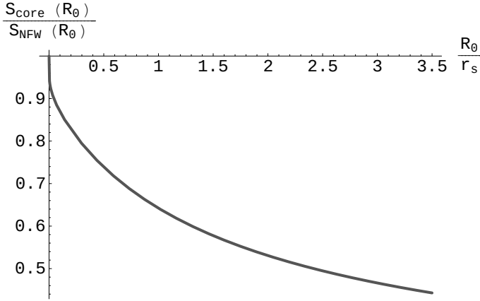
Figure 3.1: The ratio of average column densities of the extreme cored and NFW profiles as a function of R_0 (c.f. Eq. (3.15)).
