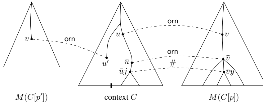
Fig. 1. \bar{u} = \text{orn}_{C[p]}(\bar{v}) is not a proper ancestor of u' = \text{orn}_{C[p']}(\bar{v})
